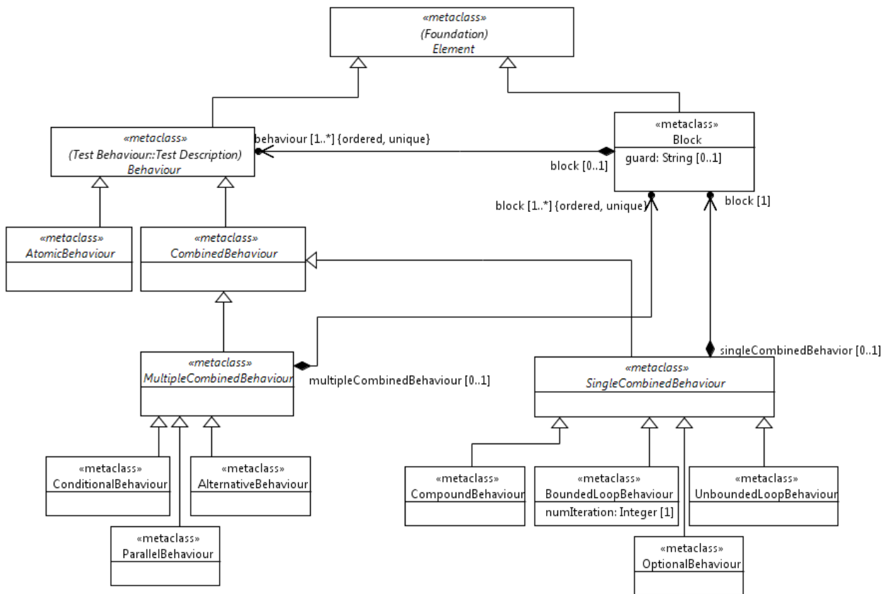
Figure 8.2: Behaviour Concepts
