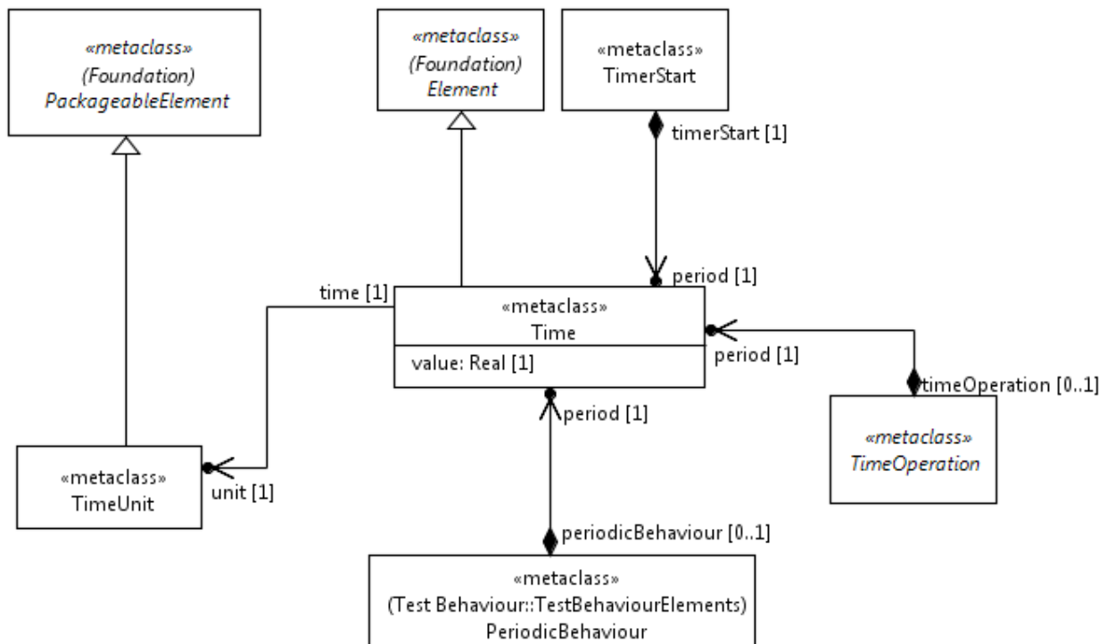
Figure 9.1: Time Concept
