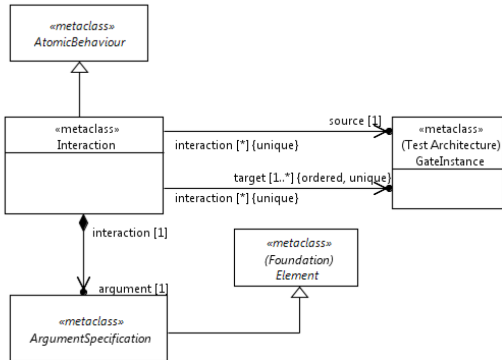
Figure 8.4: Interaction Concepts
