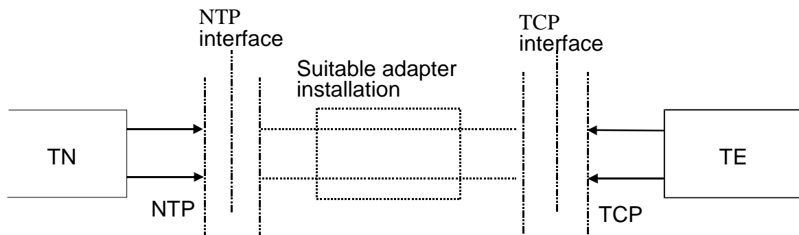
Figure 1: Terminal connection point and network termination point
