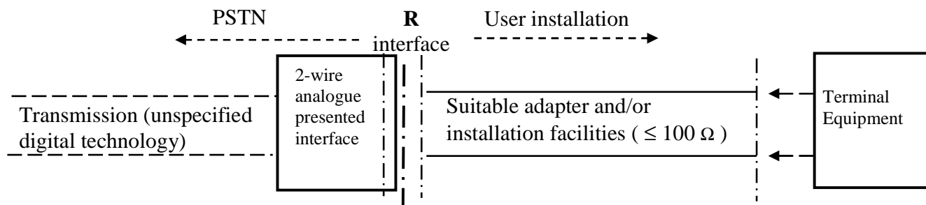
Figure 1: 2-wire analogue presented interface (R-interface)
