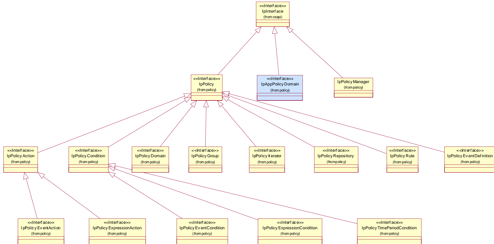
Figure 1: Policy Classes
