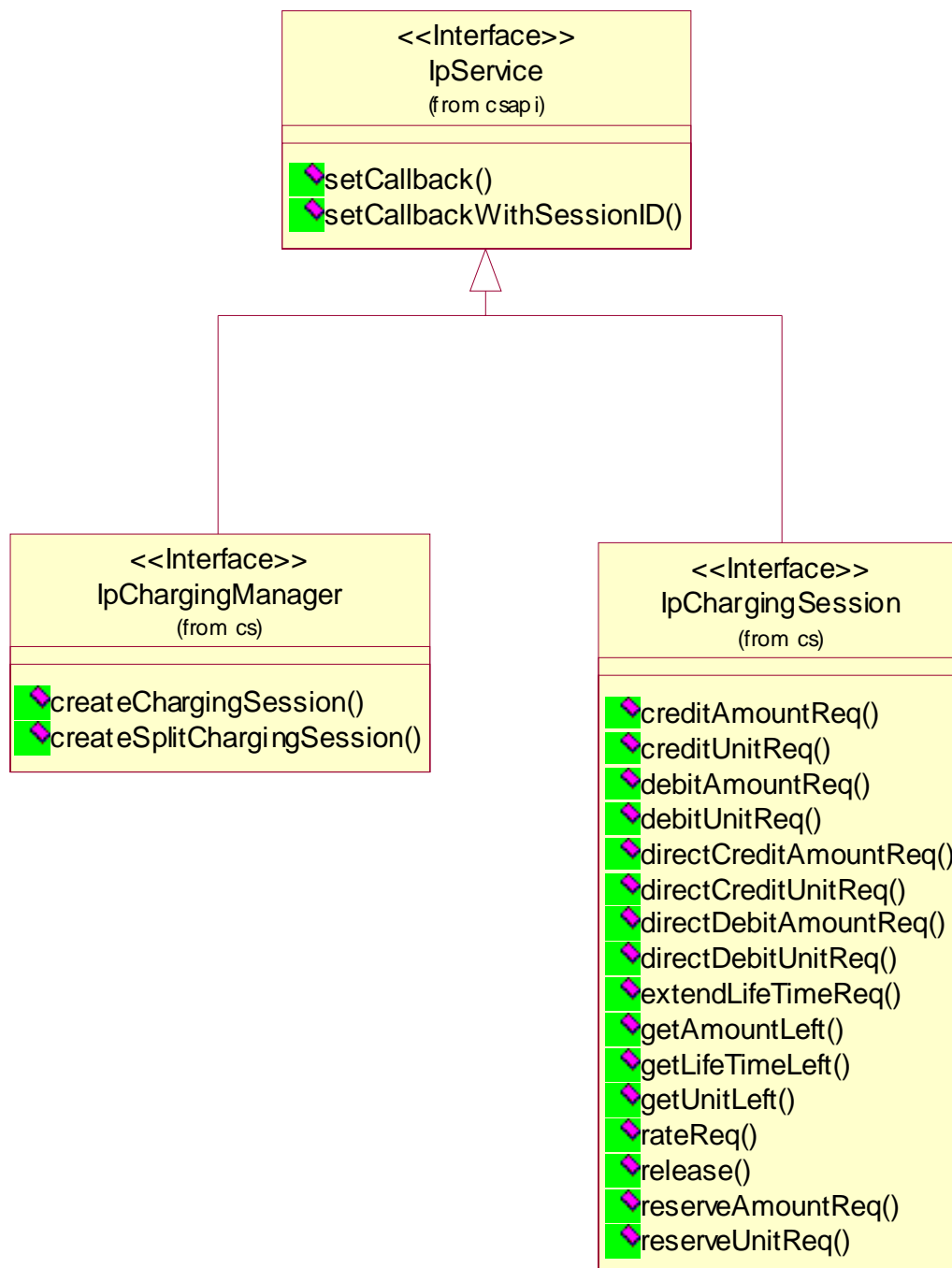
Figure 2: Service Interfaces
