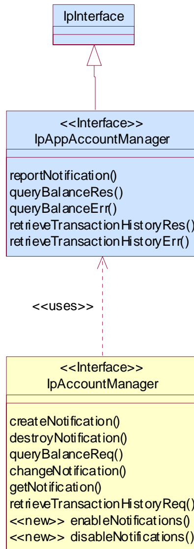
Figure 1: Application Interfaces
