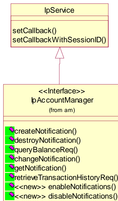
Figure 2: Service Interfaces
