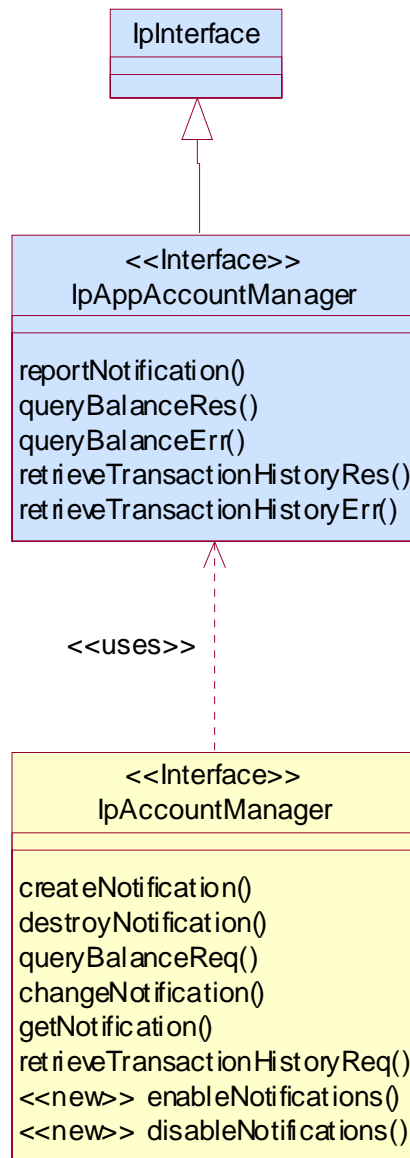
Figure 1: Application Interfaces
