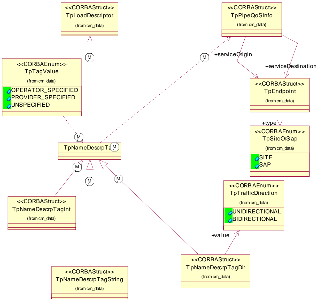
Figure 5: Pipe QoS Data Types
