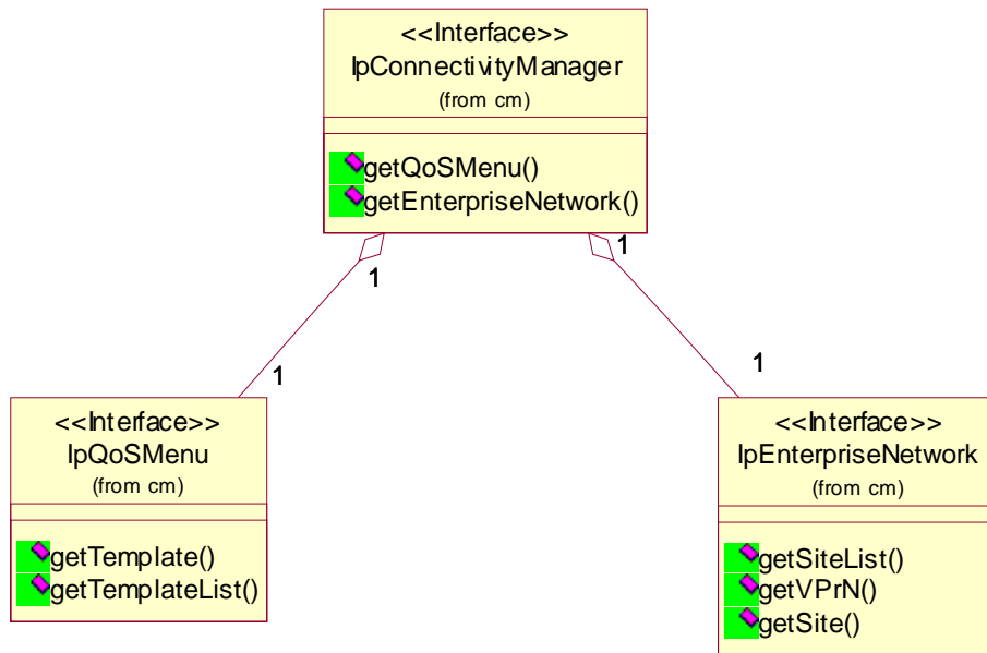
Figure 2: QoS Menu and Enterprise Network class diagram
