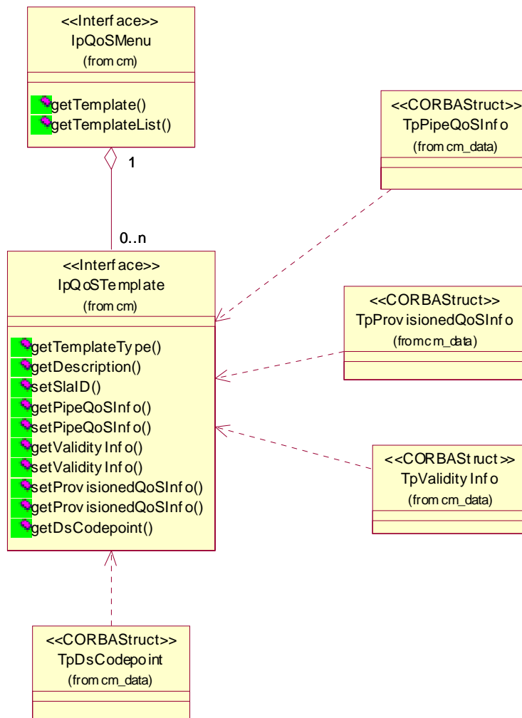
Figure 3: QoS Template class diagram
