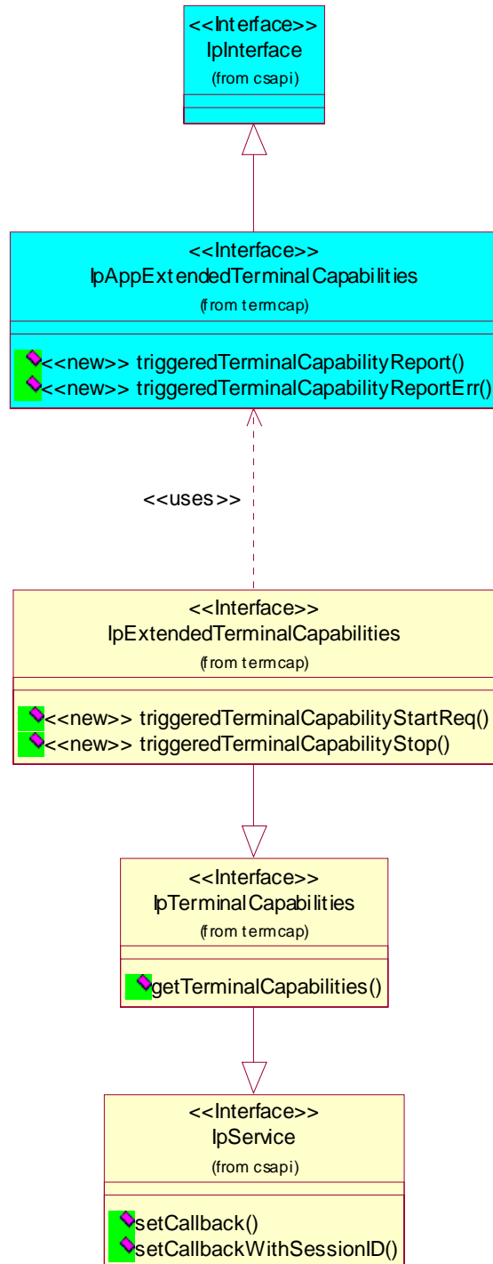
Figure 1: Terminal Capabilities Class Diagram
