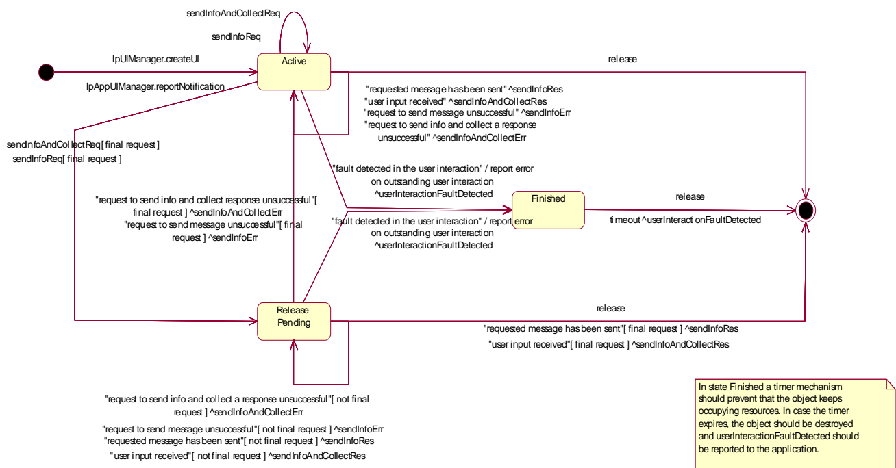
Figure 3: Application view on the UI object
