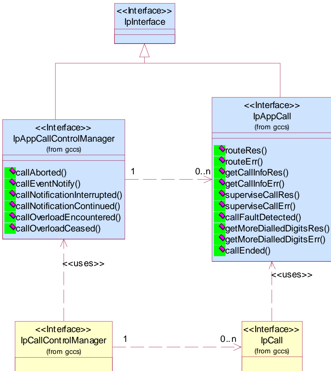
Figure 2: Application Interfaces
