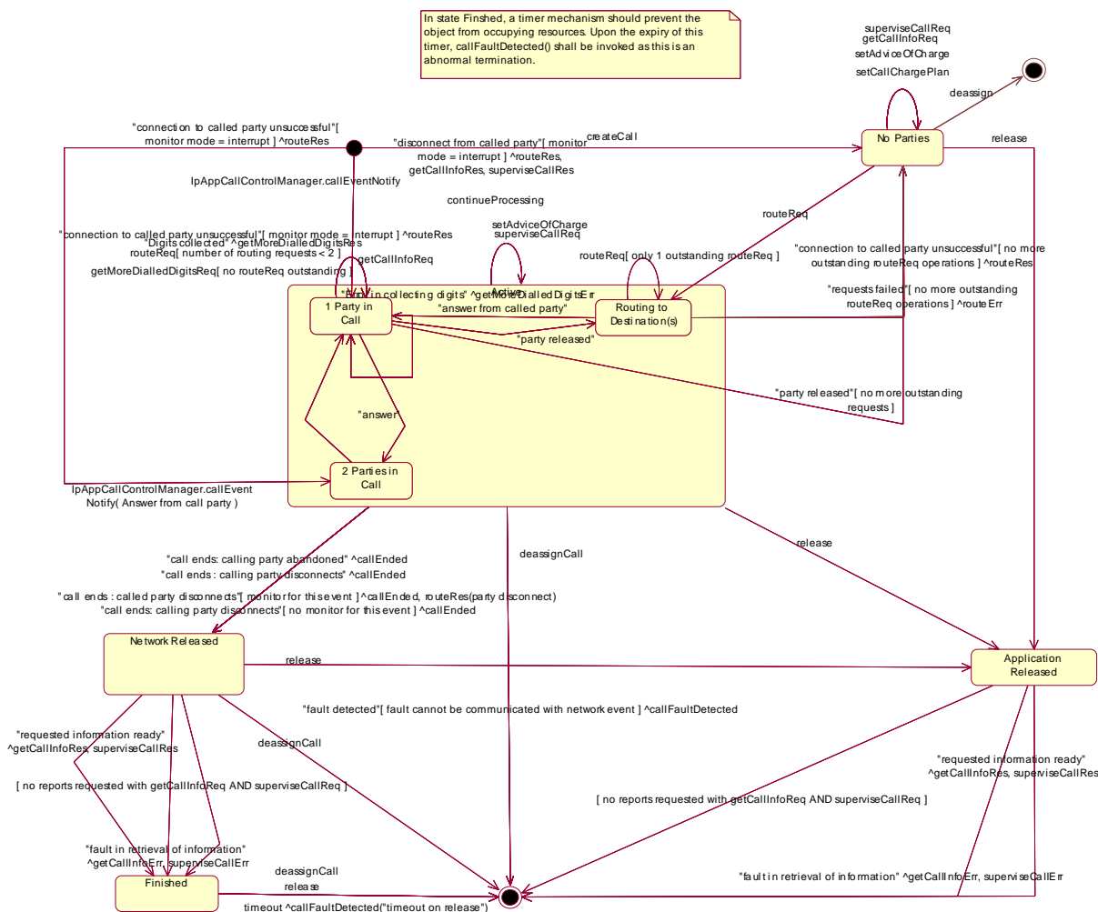
Figure 4: Application view on the IpCall object
