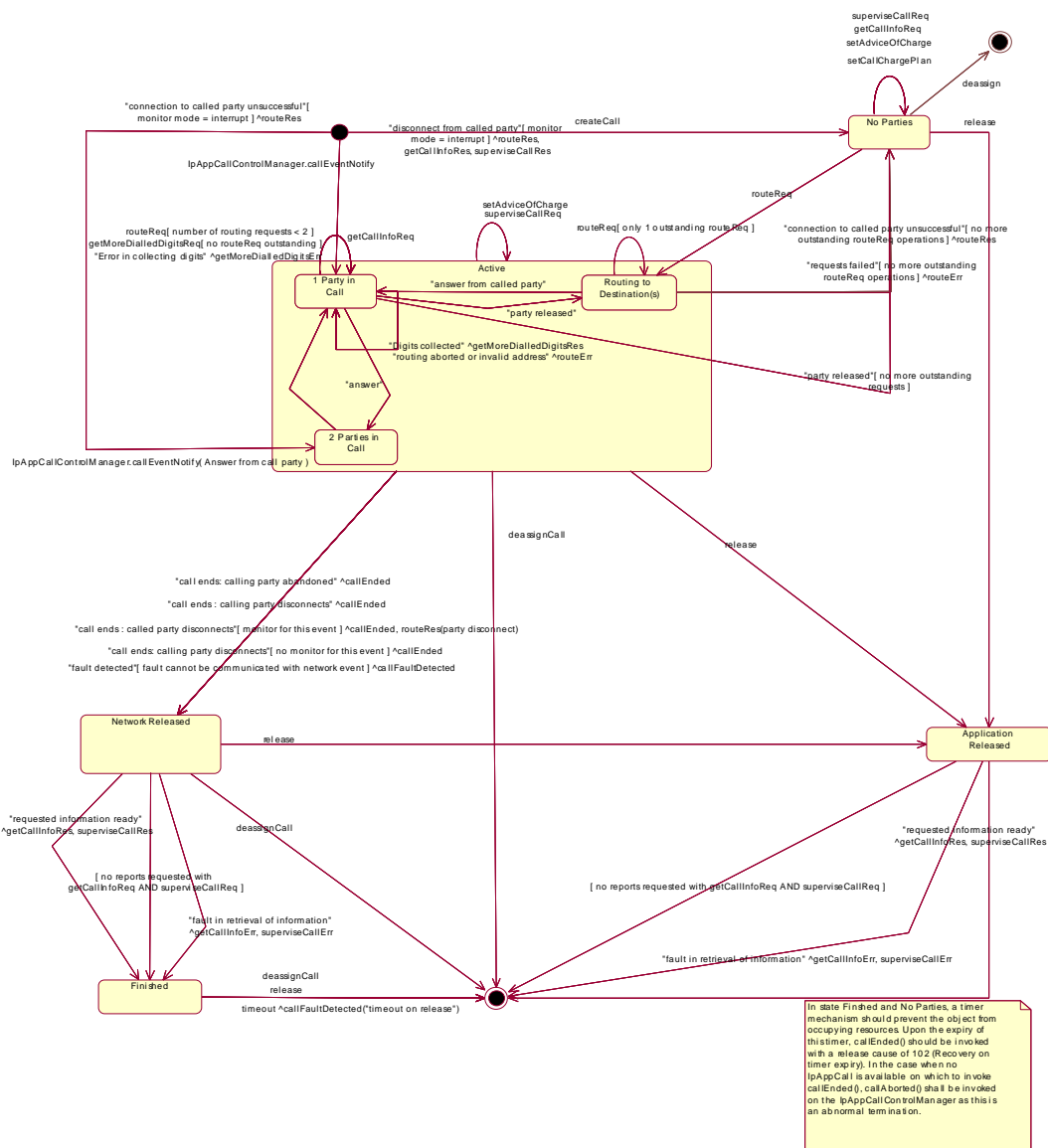
Figure 4: Application view on the IpCall object
