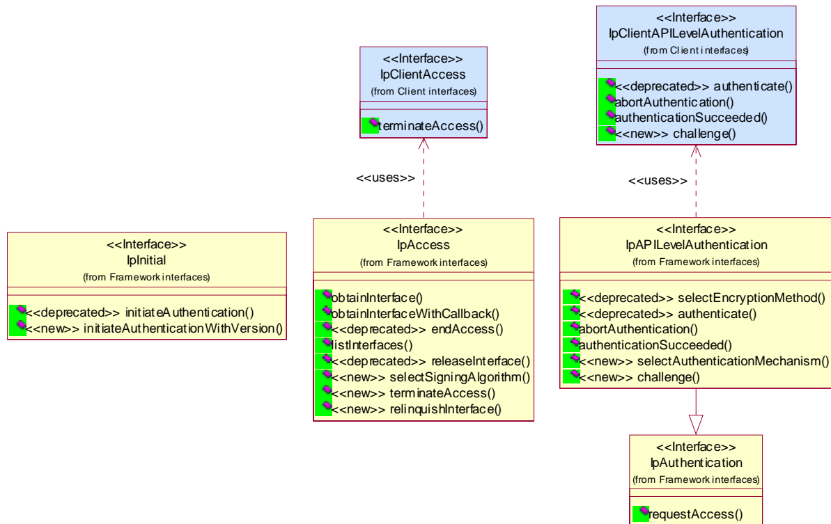
Figure 30: Trust and Security Management Package Overview
