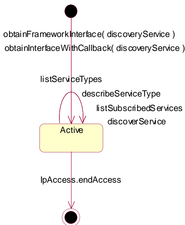
Figure 13: State Transition Diagram for IpServiceDiscovery
