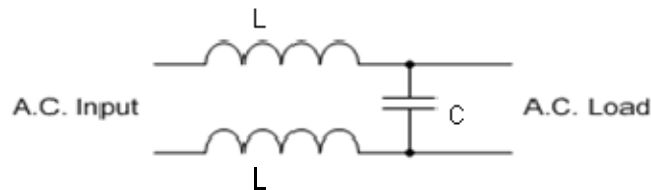
Figure 5: Example of how to improve coexistence between CPS and PLT technology
