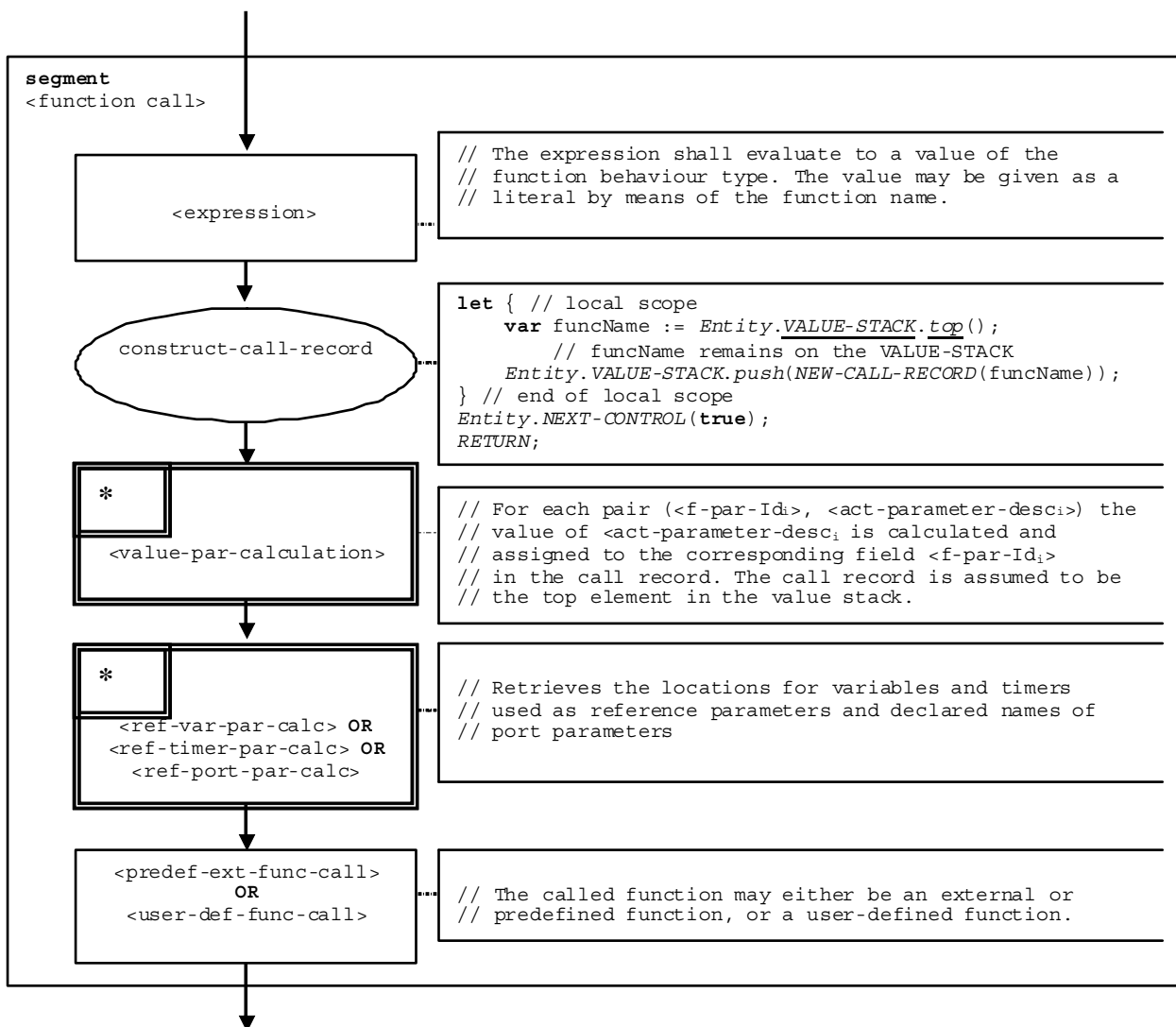
Figure 80: Flow graph segment <function-call>
