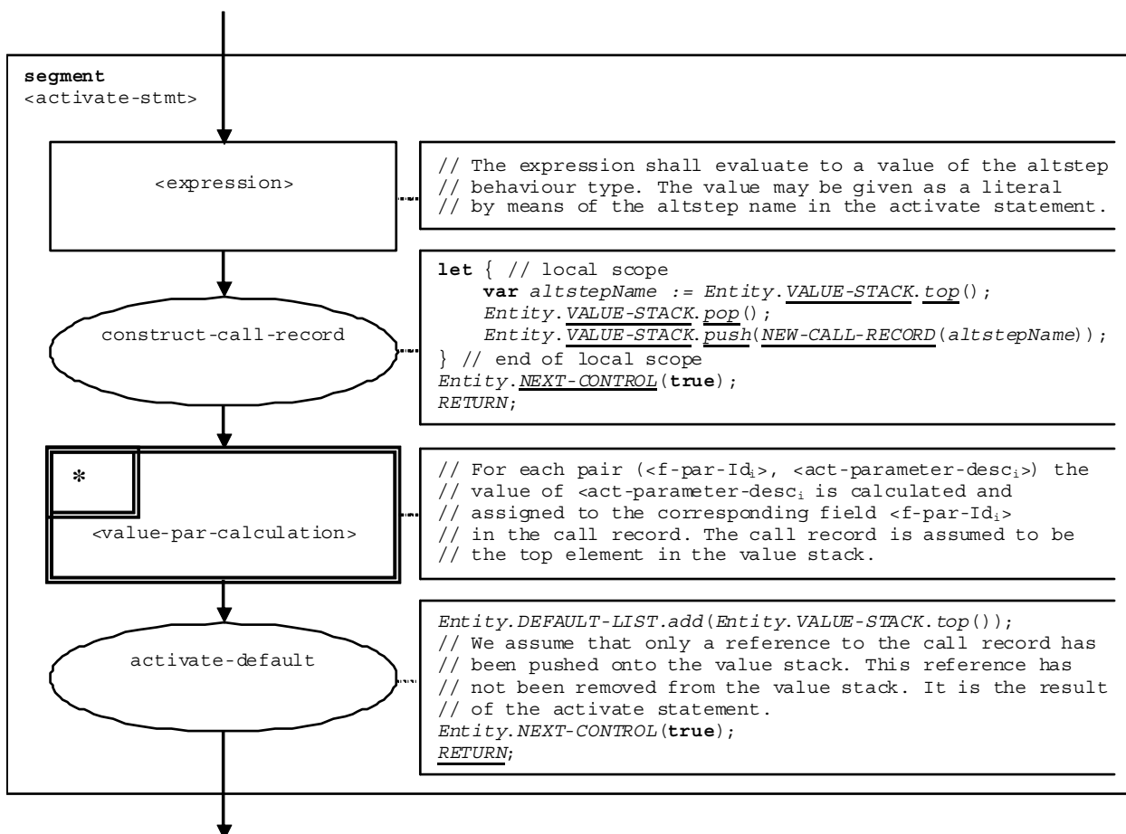
Figure 37: Flow graph segment &lt;activate-stmt&gt;
