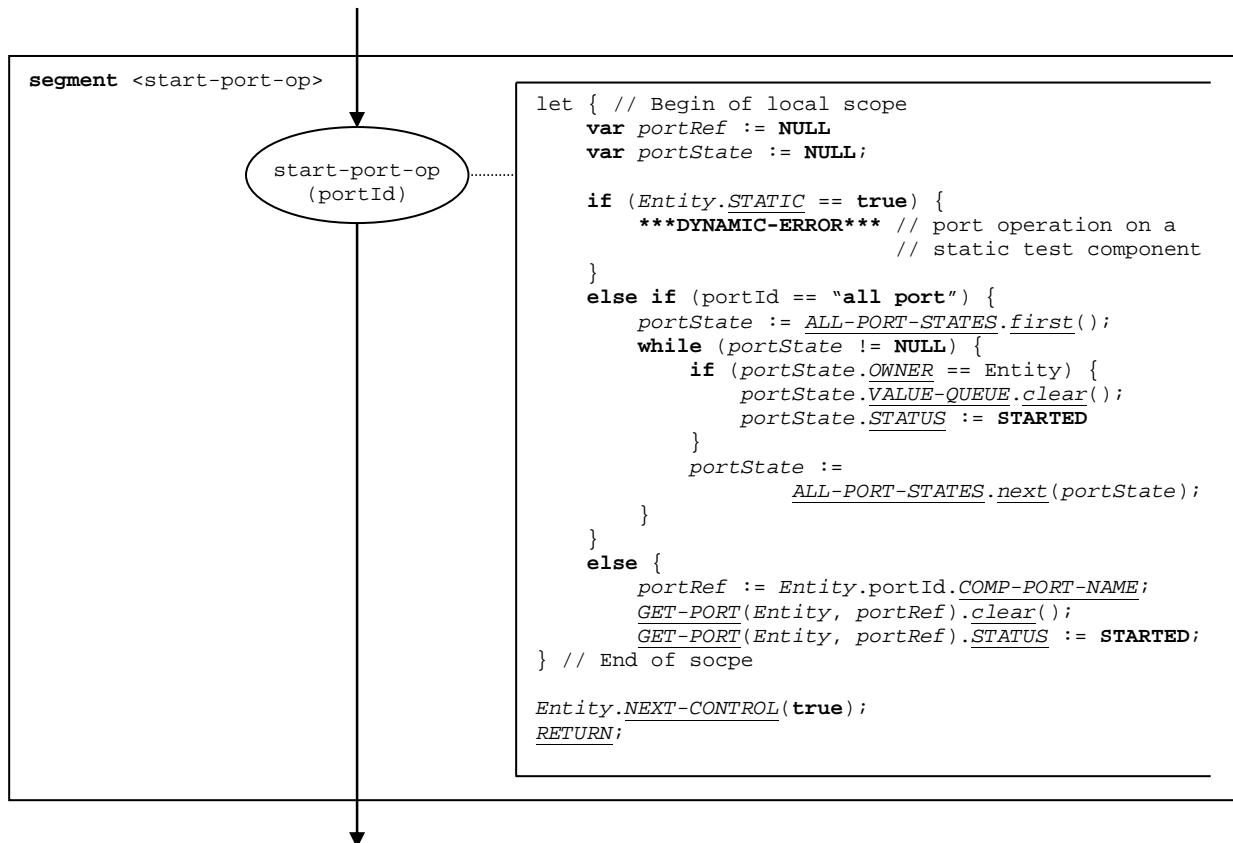
Figure 121 of ETSI ES 201 873-4 [2]: Flow graph segment <start-port-op>
