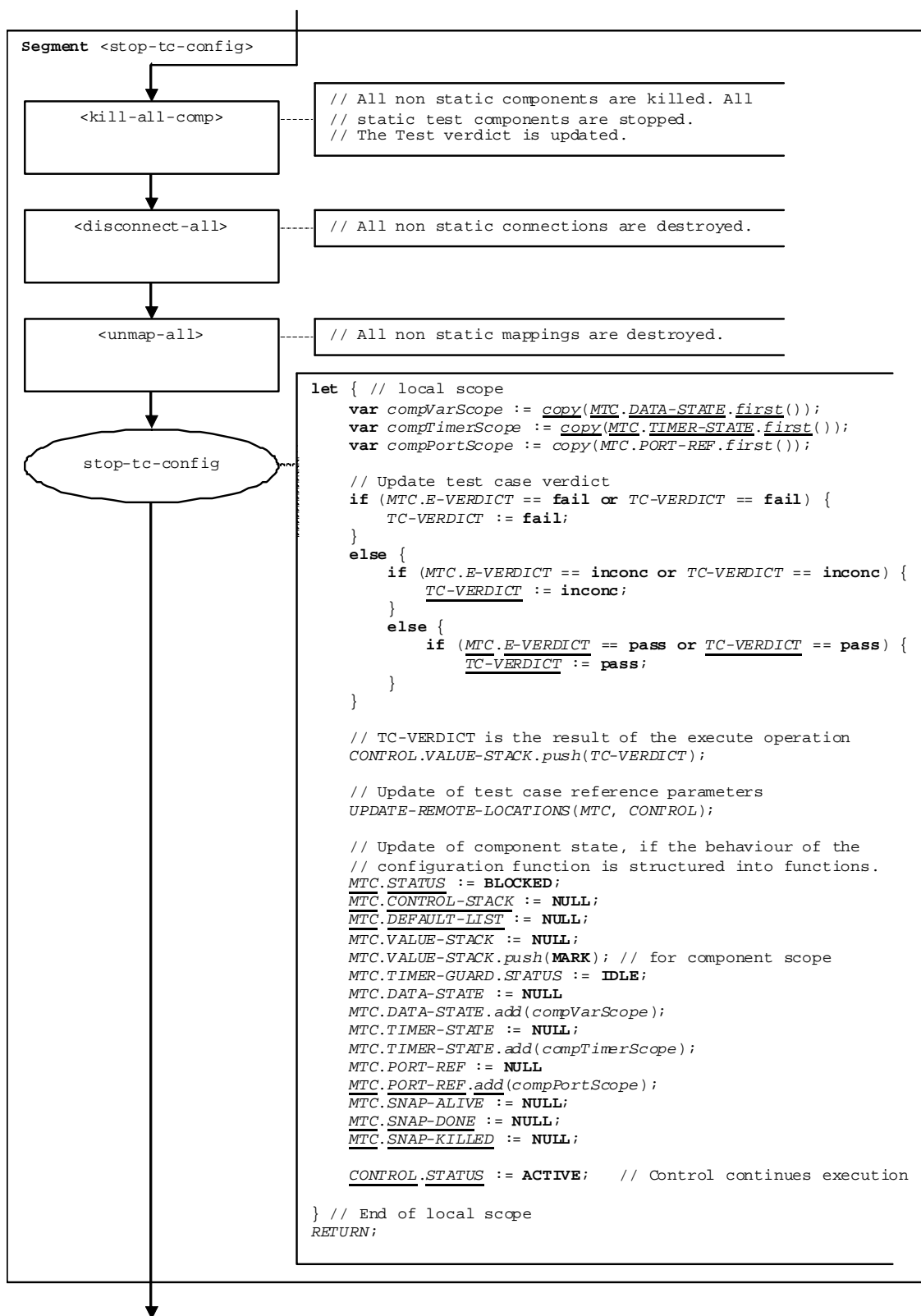
Figure 127b of ETSI ES 201 873-4 [2]: Flow graph segment &lt;stop-tc-config&gt;
