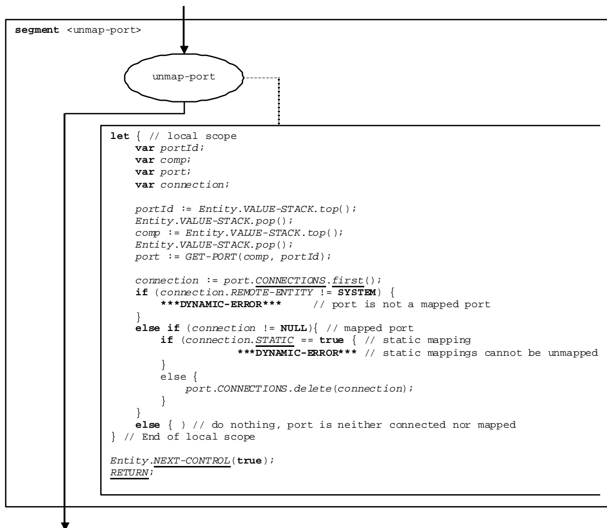
Figure 136c of ETSI ES 201 873-4 [2]: Flow graph segment <unmap-port>
