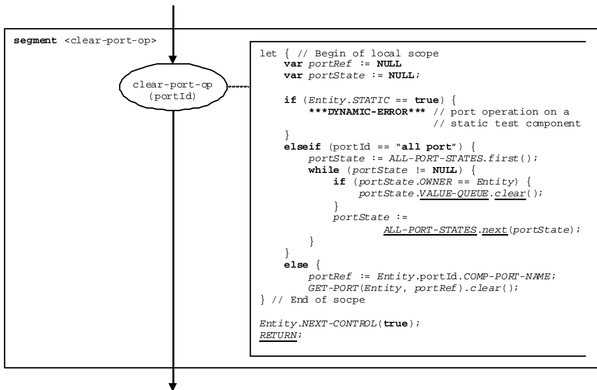
Figure 59 of ETSI ES 201 873-4 [2]: Flow graph segment <clear-port-op>
