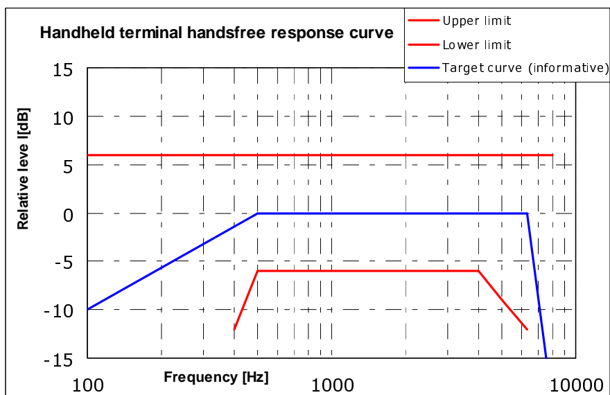
Figure 15: Receive frequency response mask for Hand-held HFT
