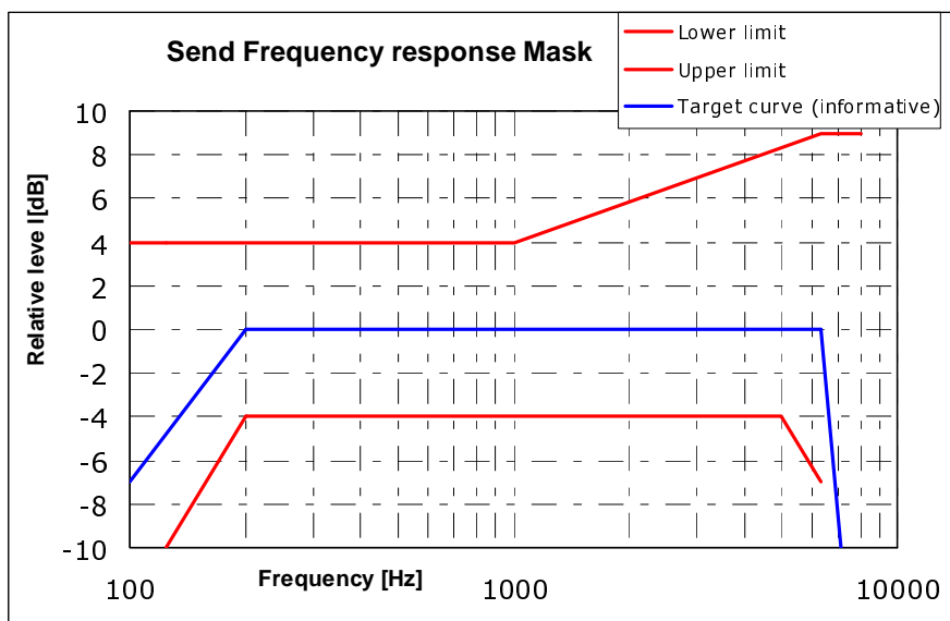
Figure 13: Sending sensitivity/frequency mask for HFT
