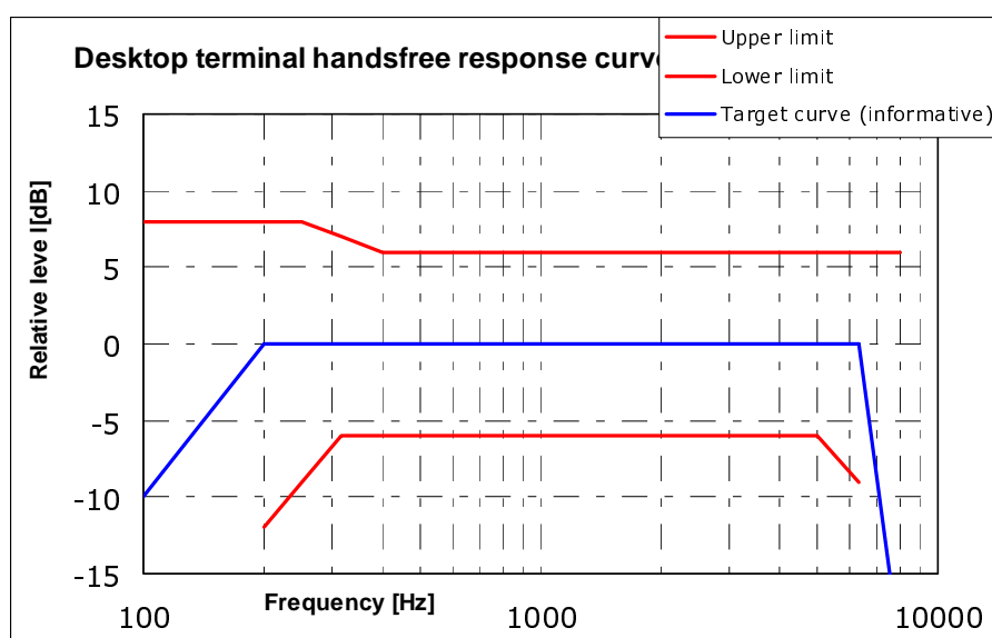
Figure 14: Receive frequency mask for Desktop HFT
