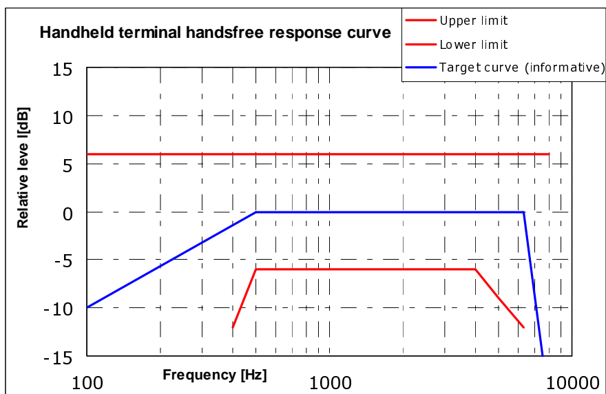
Figure 15: Receiving frequency response mask for Hand-held HFT
