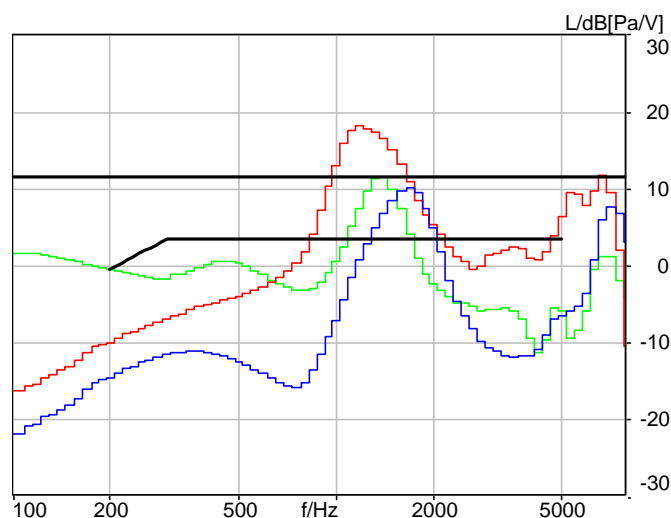
Figure B.1: Receive frequency response of 3 wideband terminals and the tolerance scheme of ETSI ES 202 739 (V1.2.1) [i.7] measured in handset mode at an artificial head, 3.4 artificial ear, free-field equalization and with 8 N application force
