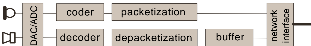
Figure A.1: Synoptic of the different functions implemented in a VoIP terminal
