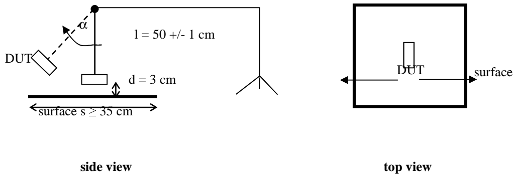
Figure 8: Positioning of handset under test
