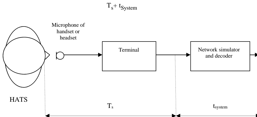
Figure 9: Different blocks contributing to the delay in send direction
