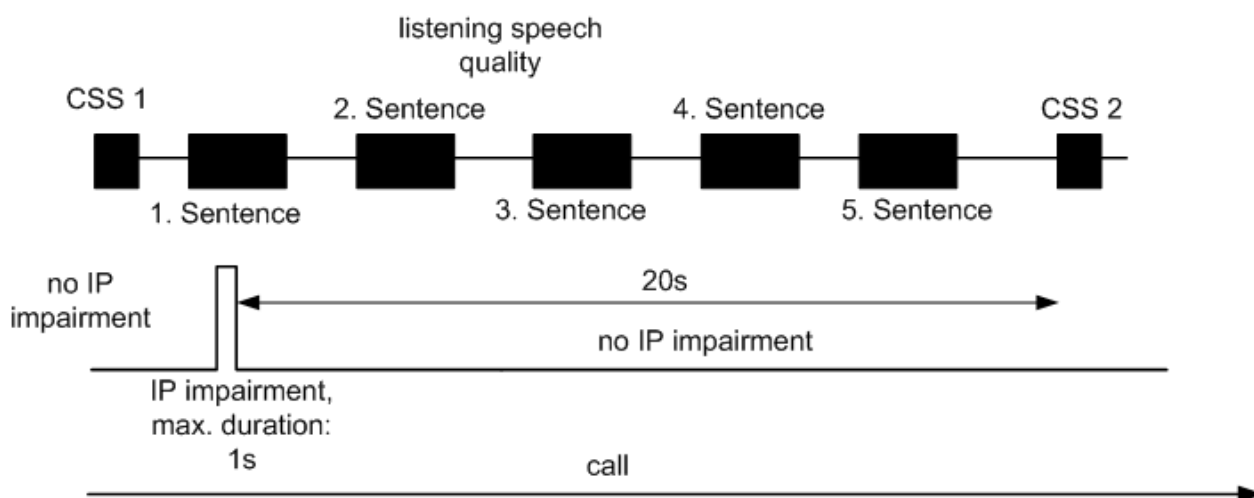
Figure 11: Test sequence to measure quality of jitter buffer adjustment (with 1 of 8 sentences)
