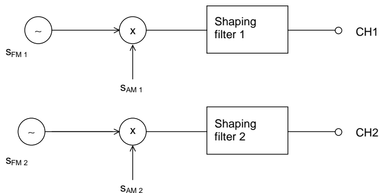
Figure 7: Measurement signals
