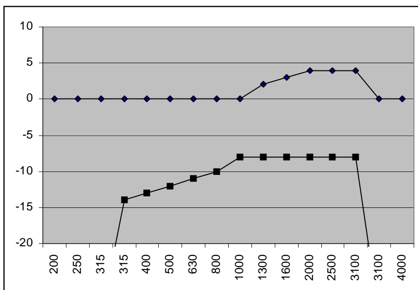
Figure 13: Sending sensitivity/frequency mask for HFT
