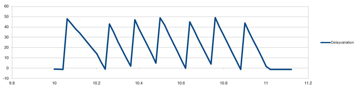
Figure C.2: Zoom in into the IP delay variation part (IPDV in ms vs. time in seconds)
