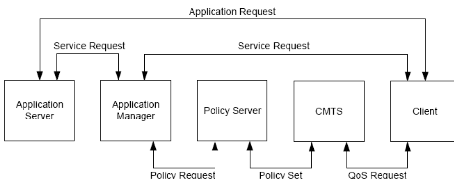
Figure B.4: Authorization Framework when Client does support native QoS mechanisms
