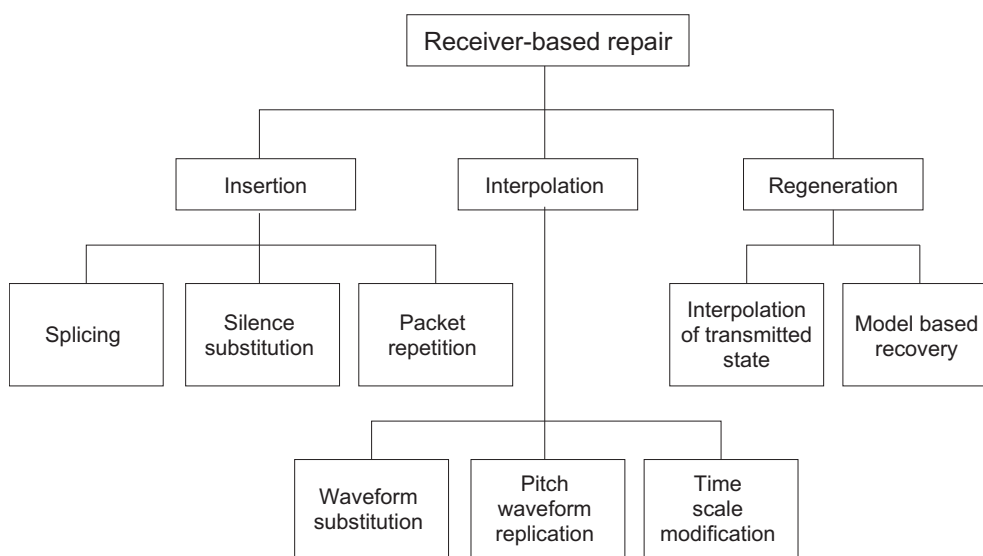
Figure C.2: A taxonomy of receiver based audio packet loss repair methods
