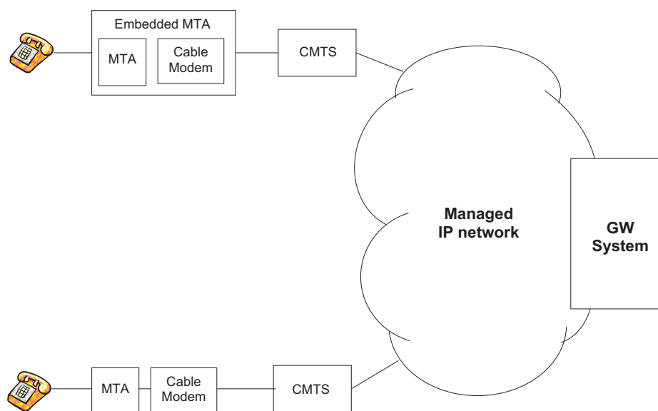
Figure 6: Cable network real-time services architecture
