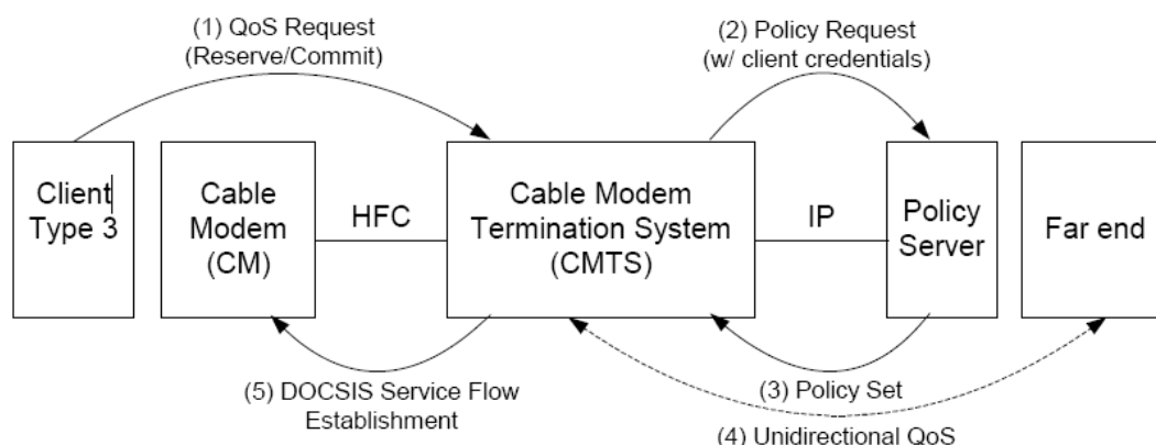
Figure B.5: Authorization Framework when Client supports RSVP
