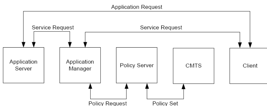
Figure B.3: Authorization Framework when Client does not support native QoS mechanisms
