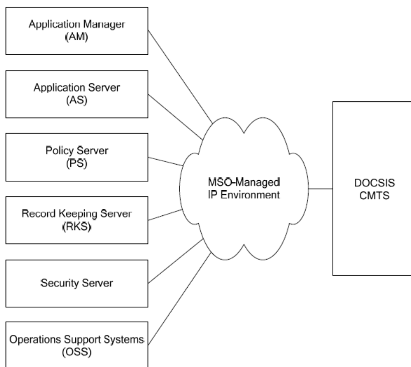
Figure B.2: Multimedia Network Elements
