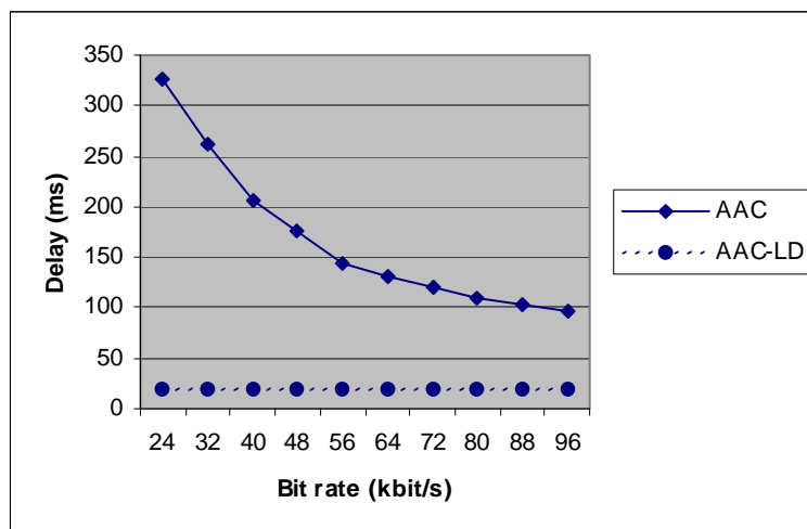
Figure 13: MPEG AAC algorithm delay
