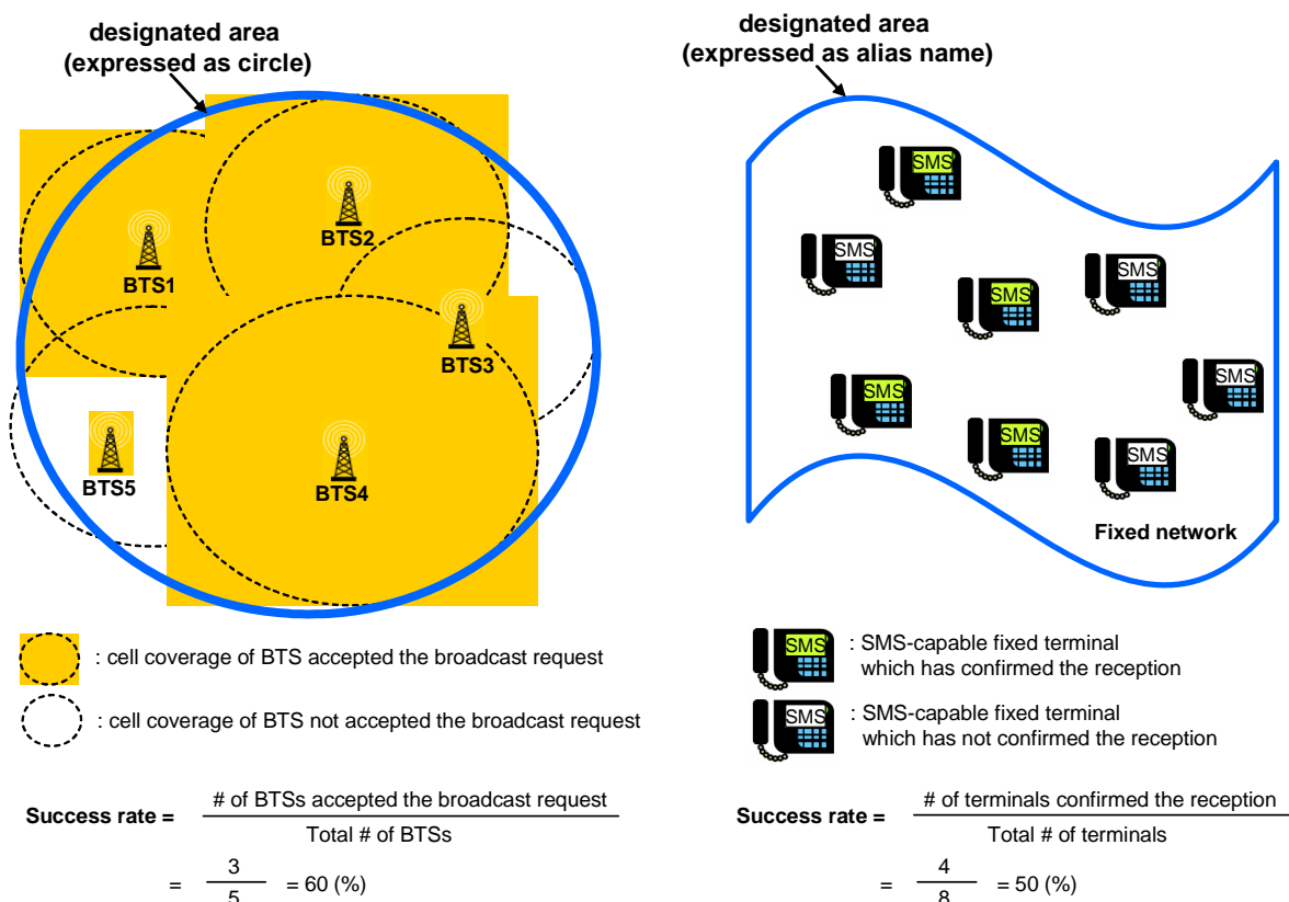
Figure 5: Success Rate
