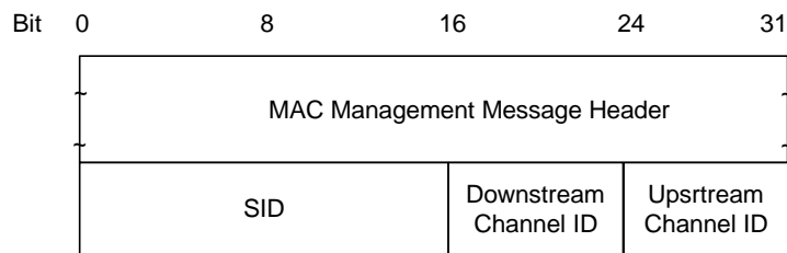
Figure 8.44: Packet PDU following the timing header
