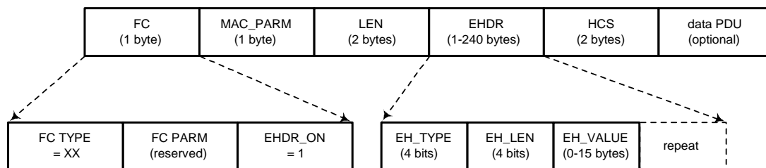
Figure 8.12: Extended MAC format
