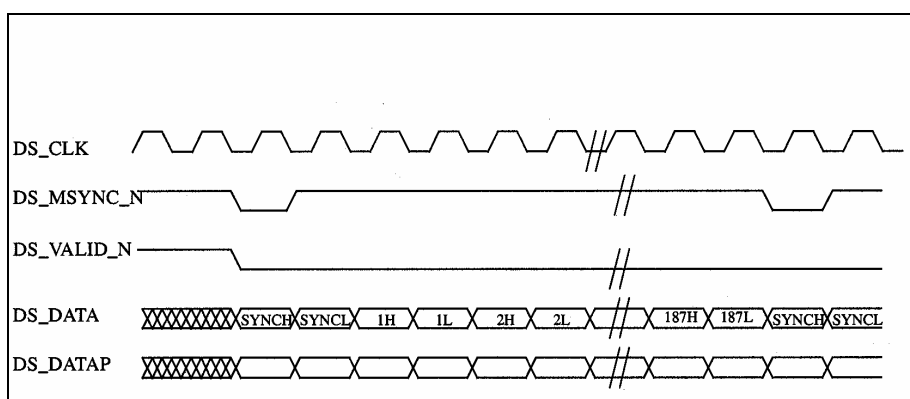
Figure H.3: Downstream data signal protocol for ITU-T Recommendation J.83 [12], annex B operation
