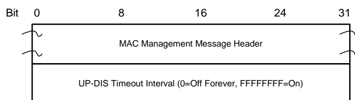
Figure 8.43: UP-DIS message format
