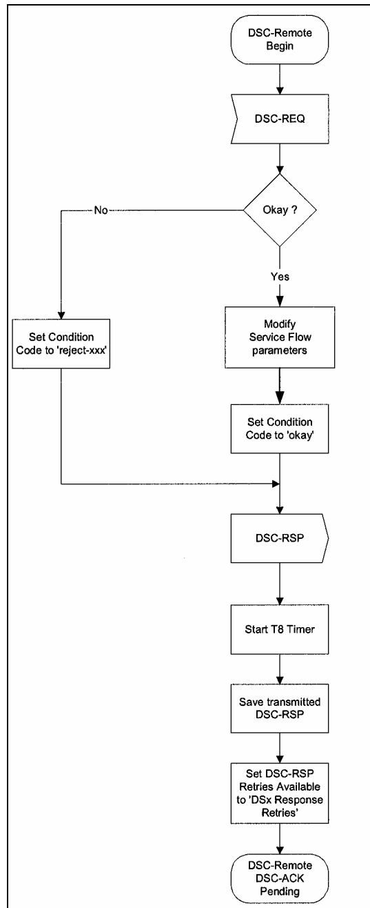
Figure 11.47: DSC-remotely initiated transaction begin state flow diagram
