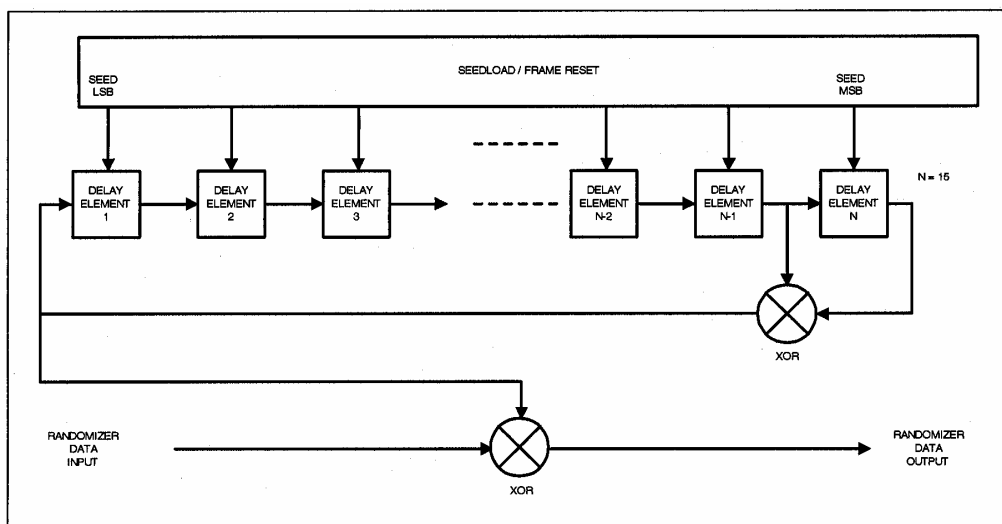
Figure 6.7: Scrambler structure
