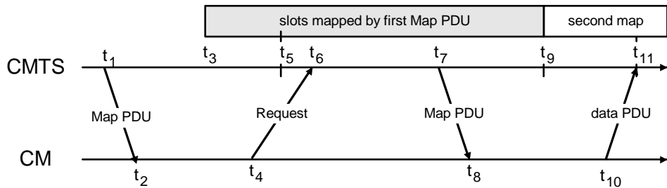
Figure 9.2: Protocol example
