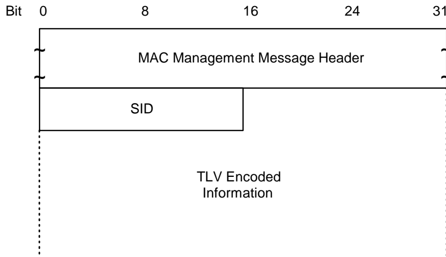
Figure 8.25: Registration - Request
