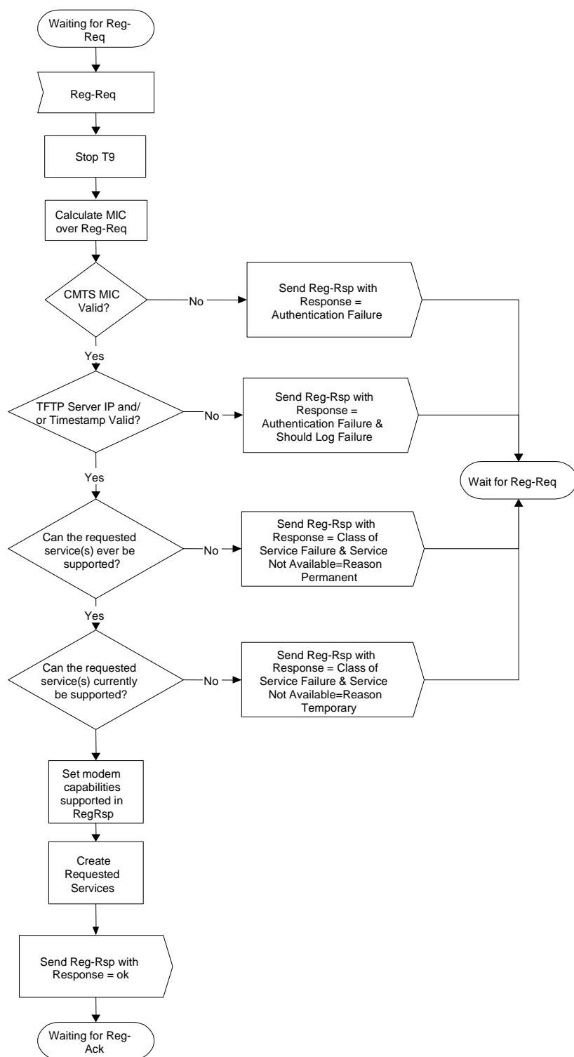
Figure 11.14: Registration - CMTS
