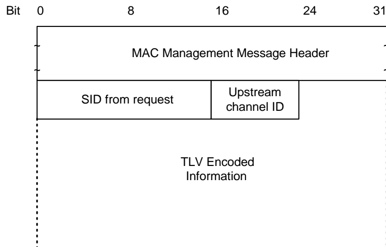
Figure 8.22: Ranging - Response
