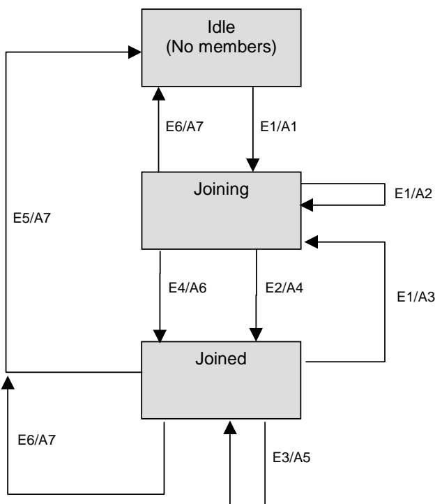
Figure O.1: IGMP support - CM passive mode
