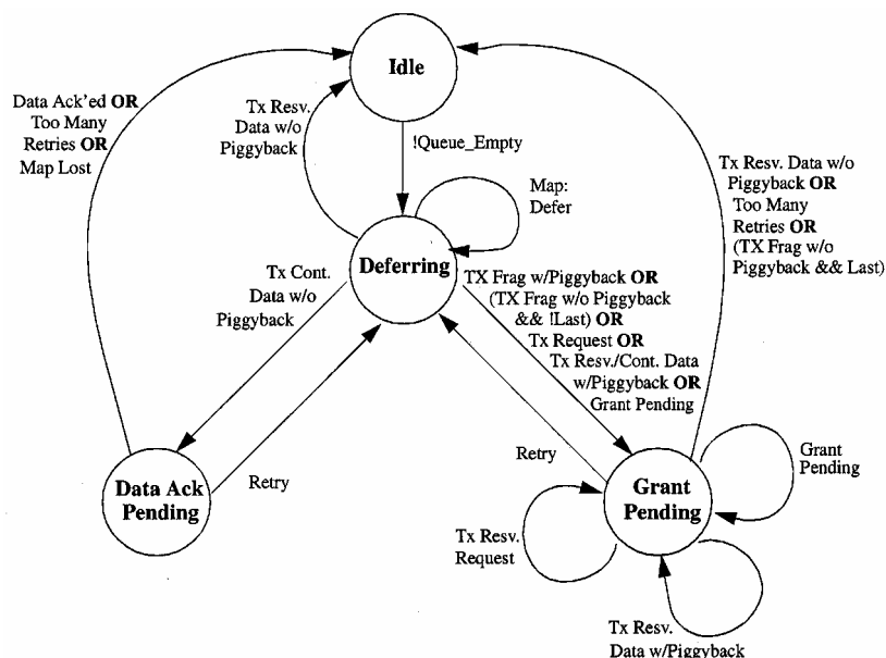
Figure N.1: Transmission and deference state transition diagram
