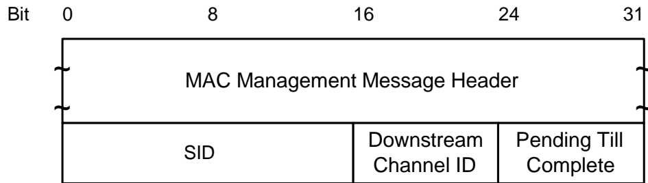
Figure 8.21: Packet PDU following the timing header
