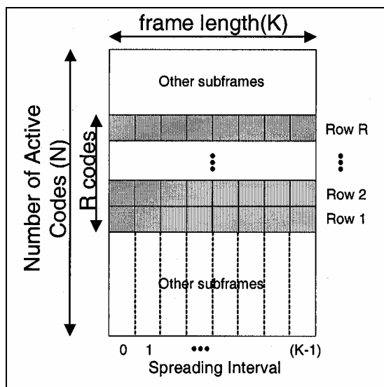
Figure 6.16: Subframe structure
