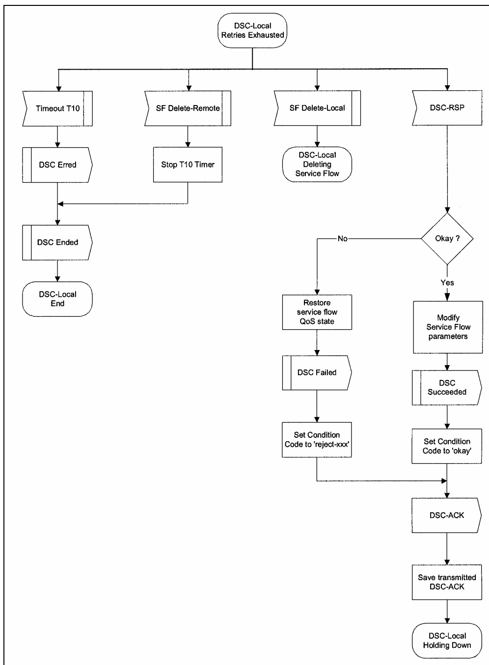
Figure 11.45: DSC-locally initiated transaction retries exhausted state flow diagram
