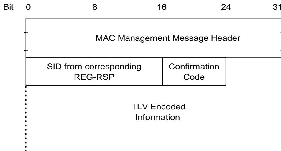
Figure 8.27: Registration - Acknowledgment
