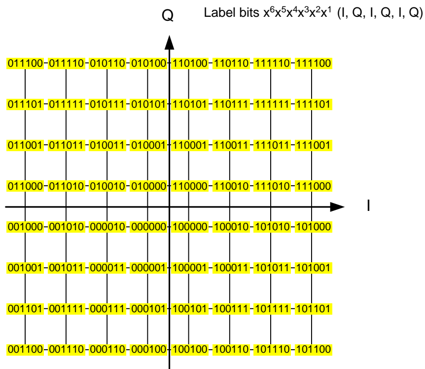
Figure 6.23: 64 QAM symbol mapping
