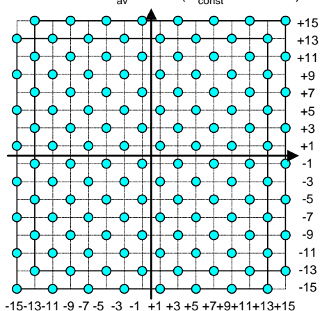
Figure 6.18: Symbol constellations
