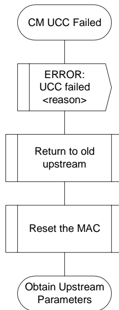
Figure 11.20: Changing upstream channels: CM view part 2
