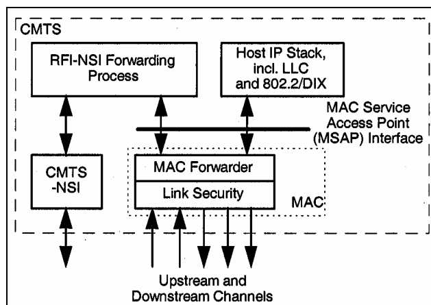
Figure 5.4: MAC forwarder
