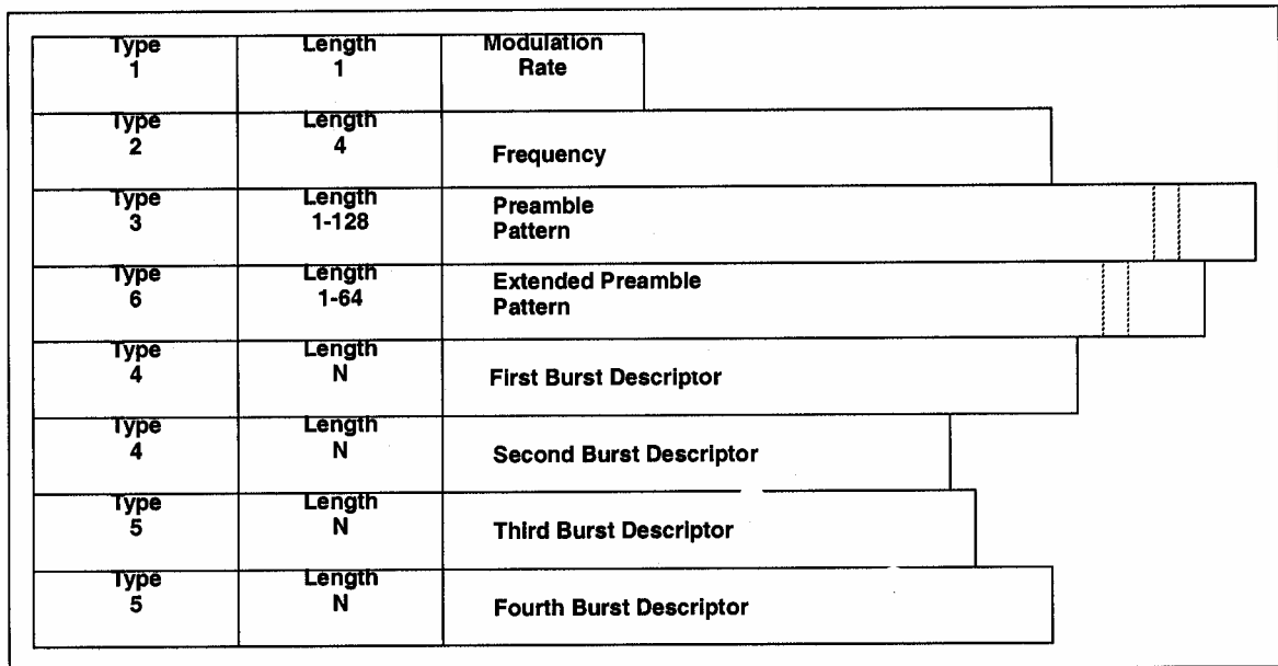
Figure 8.18: Example of UCD encoded TLV data
