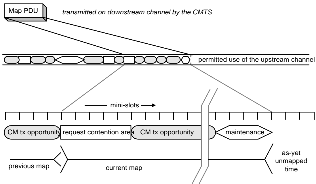
Figure 9.1: Allocation map
