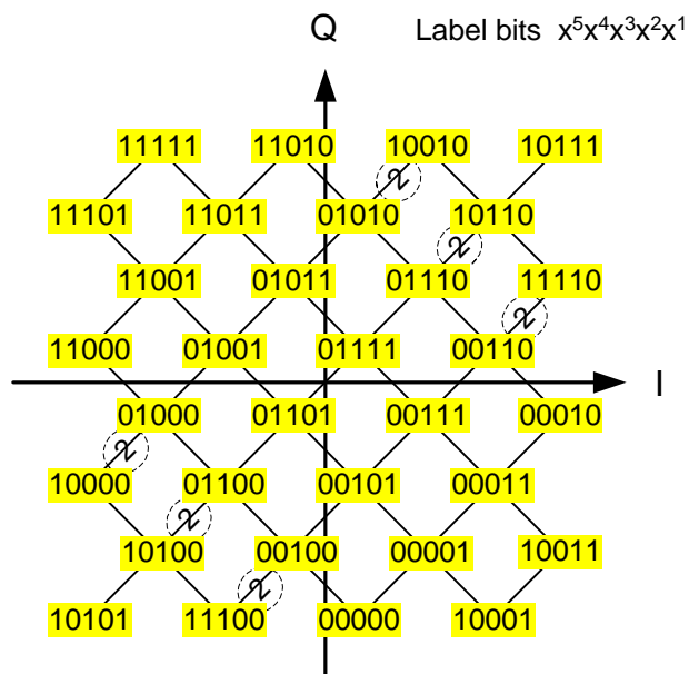
Figure 6.22: 32 QAM symbol mapping
