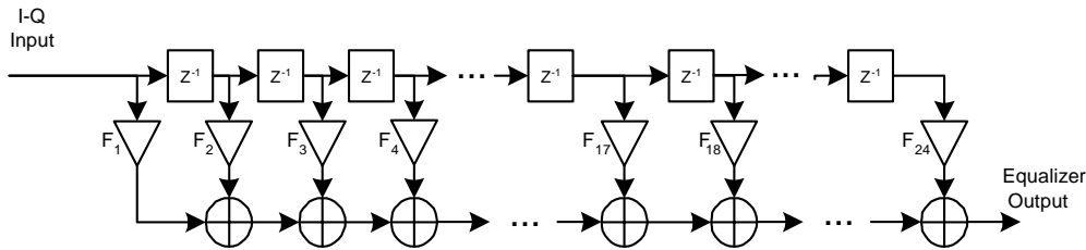
Figure 6.28: Transmit pre-equalizer structure
