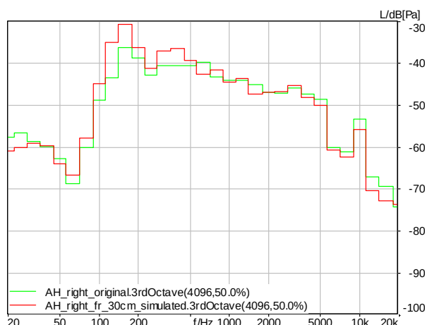
Figure 14: Original (green curve) and simulated power density spectra measured at the right ear of the artificial head
