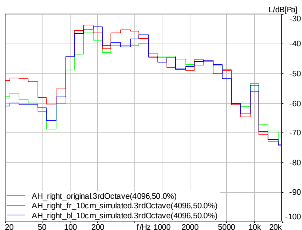
Figure 12: Original (green curve) and simulated power density spectra measured at the right ear of the artificial head
