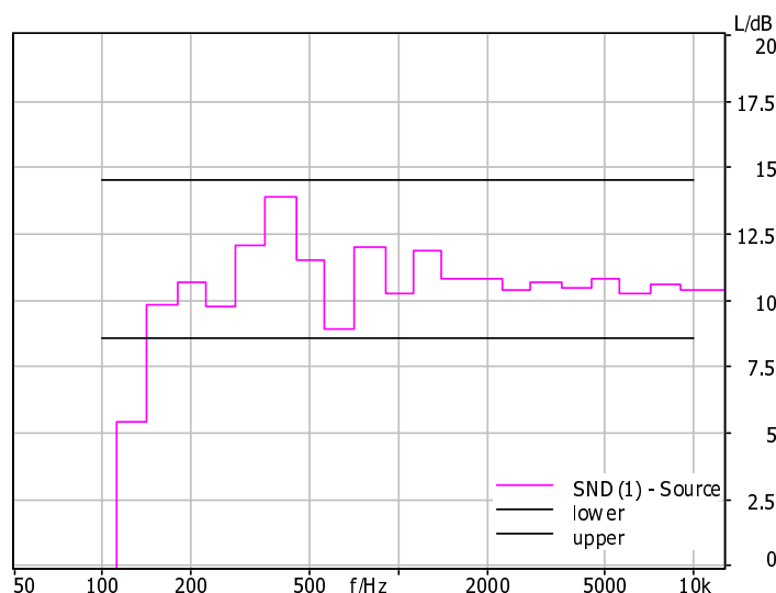
Figure 33: Difference of the original signal and the equalized signal reproduced by the front-left loudspeaker measured with the left cardioid microphone (without subwoofer)
