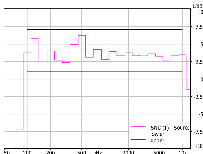
Figure 5: Difference of the original signal and the equalized signal reproduced by the front-left loudspeaker measured with the artificial heads left ear (without subwoofer)
