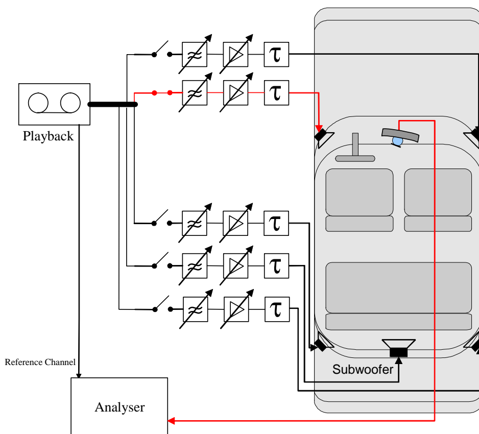
Figure 27: Block diagram of equalization setup
