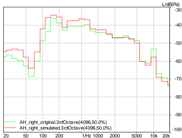
Figure 10: Power density spectra measured at the artificial heads right ear
