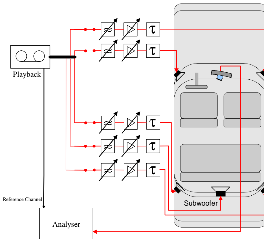
Figure 30: Block diagram of equalization setup
