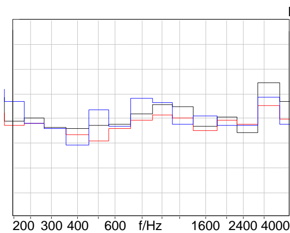
Figure B.7: Measurements of phone 7: black-fully anechoic; red - office type room; blue - semi anechoic
