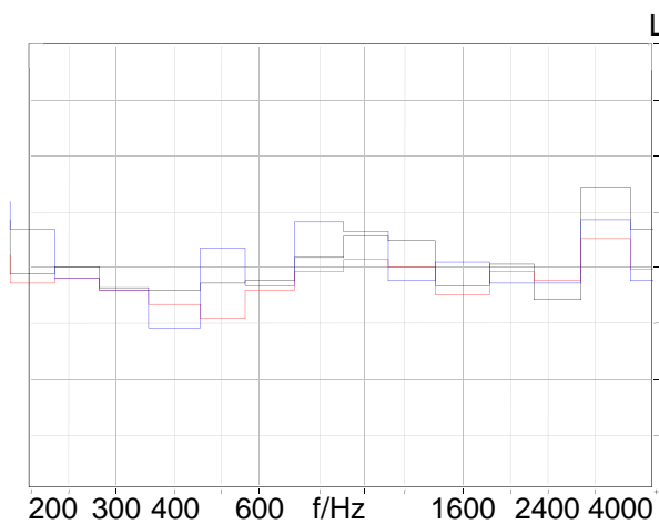
Figure B.7: Measurements of phone 7: black-fully anechoic; red - office type room; blue - semi anechoic
