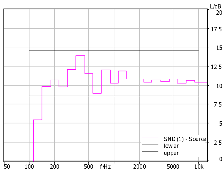
Figure 33: Difference of the original signal and the equalized signal played back by the front-left loudspeaker measured with the left cardioid microphone (without subwoofer)
