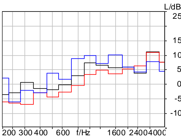
Figure B.4: Measurements of phone 4: black-fully anechoic; red - office type room; blue - semi anechoic
