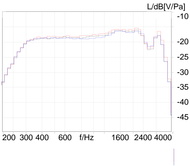
D-Value, Pink Noise
