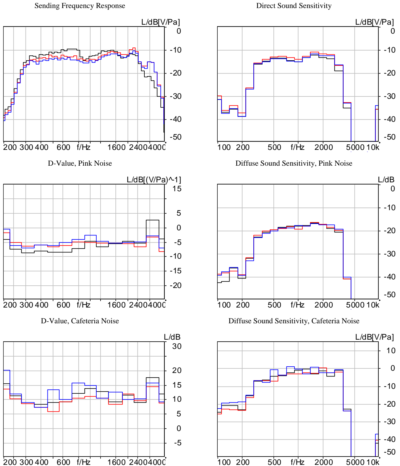
Figure B.2: Measurements of phone 2: black-fully anechoic; red - office type room; blue - semi anechoic
