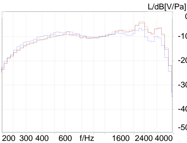
Sending Frequency Response
