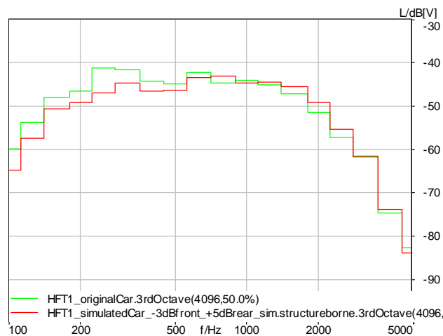
Figure 37: Power density spectra measured with a common hands-free terminal (with background noise signal processing) positioned at the ceiling near the rear-view mirror
