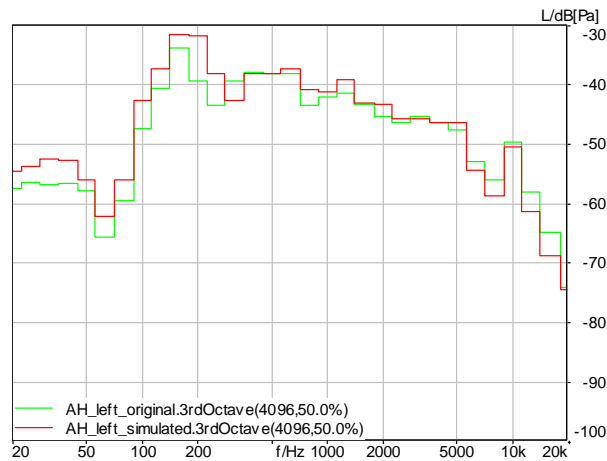
Figure 9: Power density spectra measured at the artificial heads left ear
