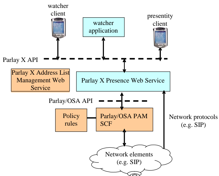
Figure 1: Presence web service environment
