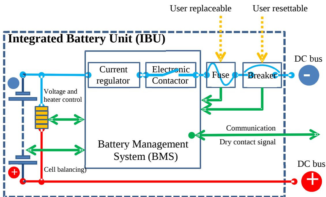
Figure 1: Functional schematic example of an IBU
