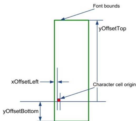
Figure 13.2: Font Bounds
