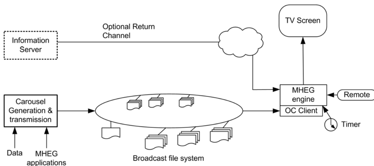
Figure 5.1: Basic Architecture
