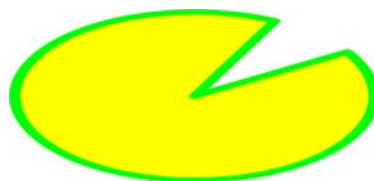
Figure 12.8: DrawSector illustrated
