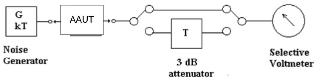
Figure 2: Measurement arrangement
