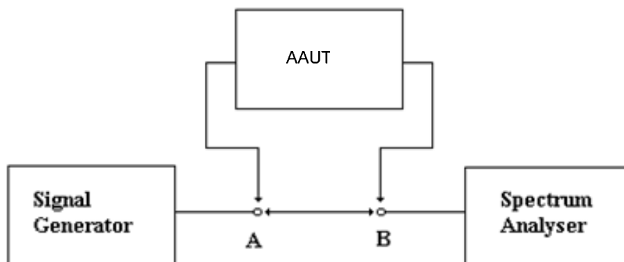
Figure 1: Measurement arrangement
