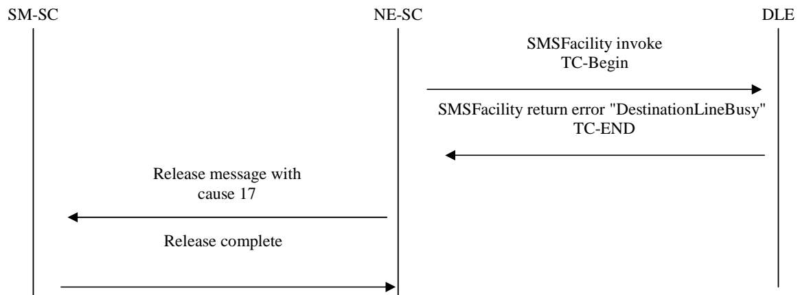
Figure A.7: Unsuccessful delivery of SMS. The SM-SC has no SCCP capabilities and is connected to the network behind a local exchange via SS7 or DSS1. Line of user B is busy.
