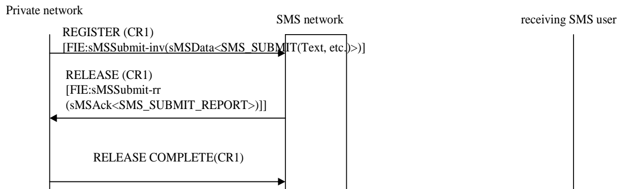
Figure A.10: Sending of a SM from a SMS originating user within a private network to the SMS network
