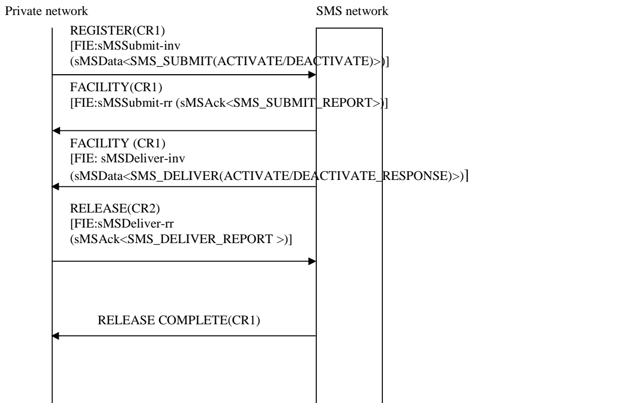
Figure A.8: Activation and Deactivation of the SMS service where the SMS user is within a private network
