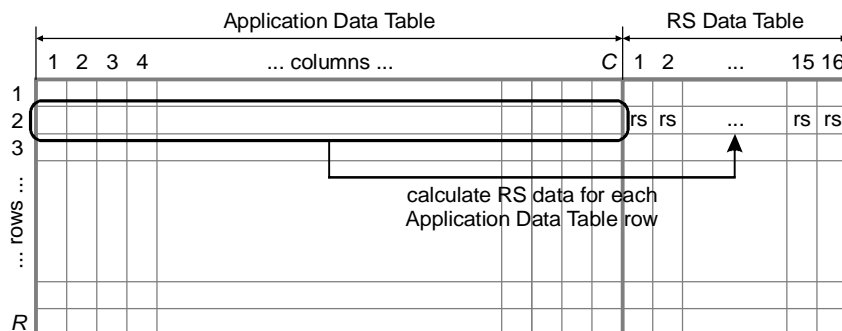
Figure 21: Calculating Reed-Solomon parity data
