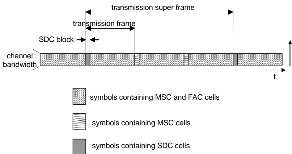
Figure 39: Time-frequency location of FAC and SDC signals
