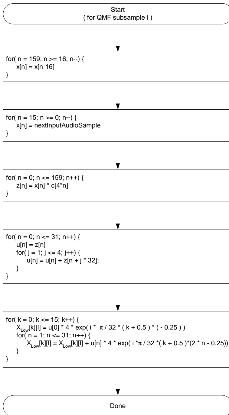
Figure 13: Flowchart of decoder 16-channel analysis QMF bank
