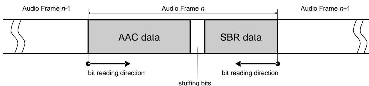
Figure 4: AAC + SBR frame
