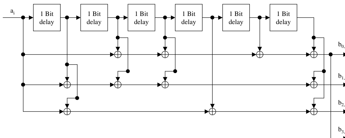
Figure 31: Convolutional encoder
