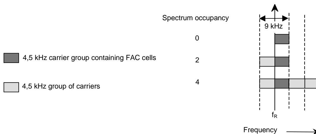
Figure 37: Spectrum occupancy for 9 kHz channels
