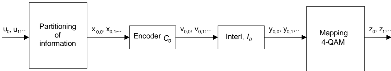
Figure 30: Multilevel coding with 1 level (SM)
