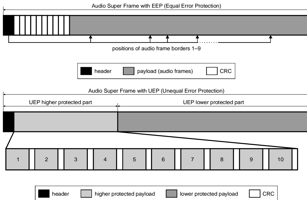
Figure 3: Example AAC audio super frame with 10 audio frames
