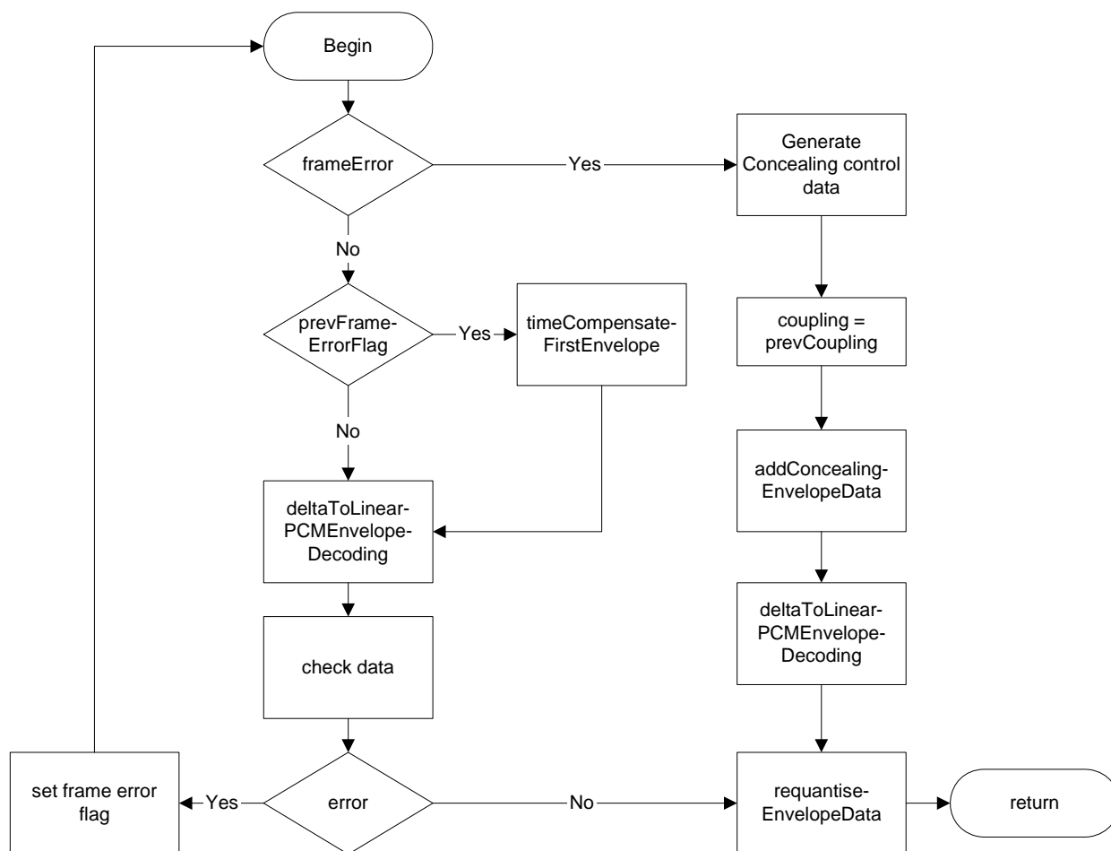
Figure 15: SBR error concealment overview
