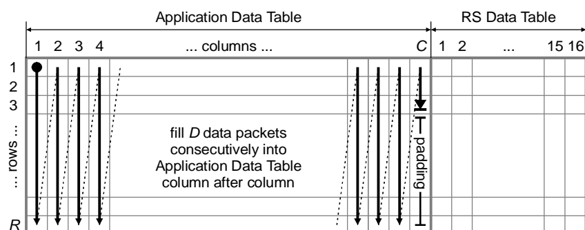
Figure 20: Placing data packets into FEC frame
