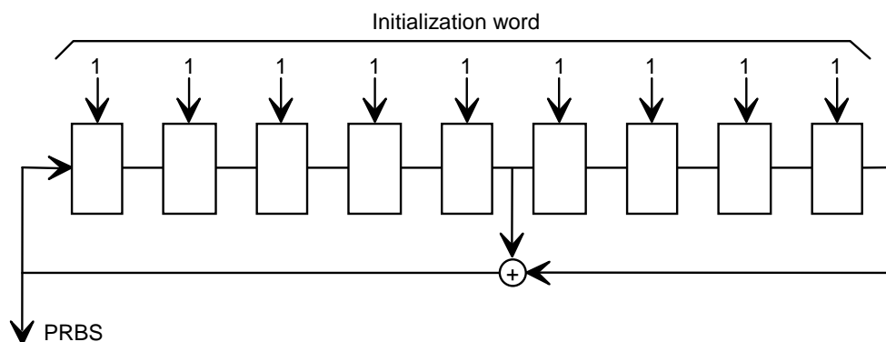
Figure 25: PRBS generator
