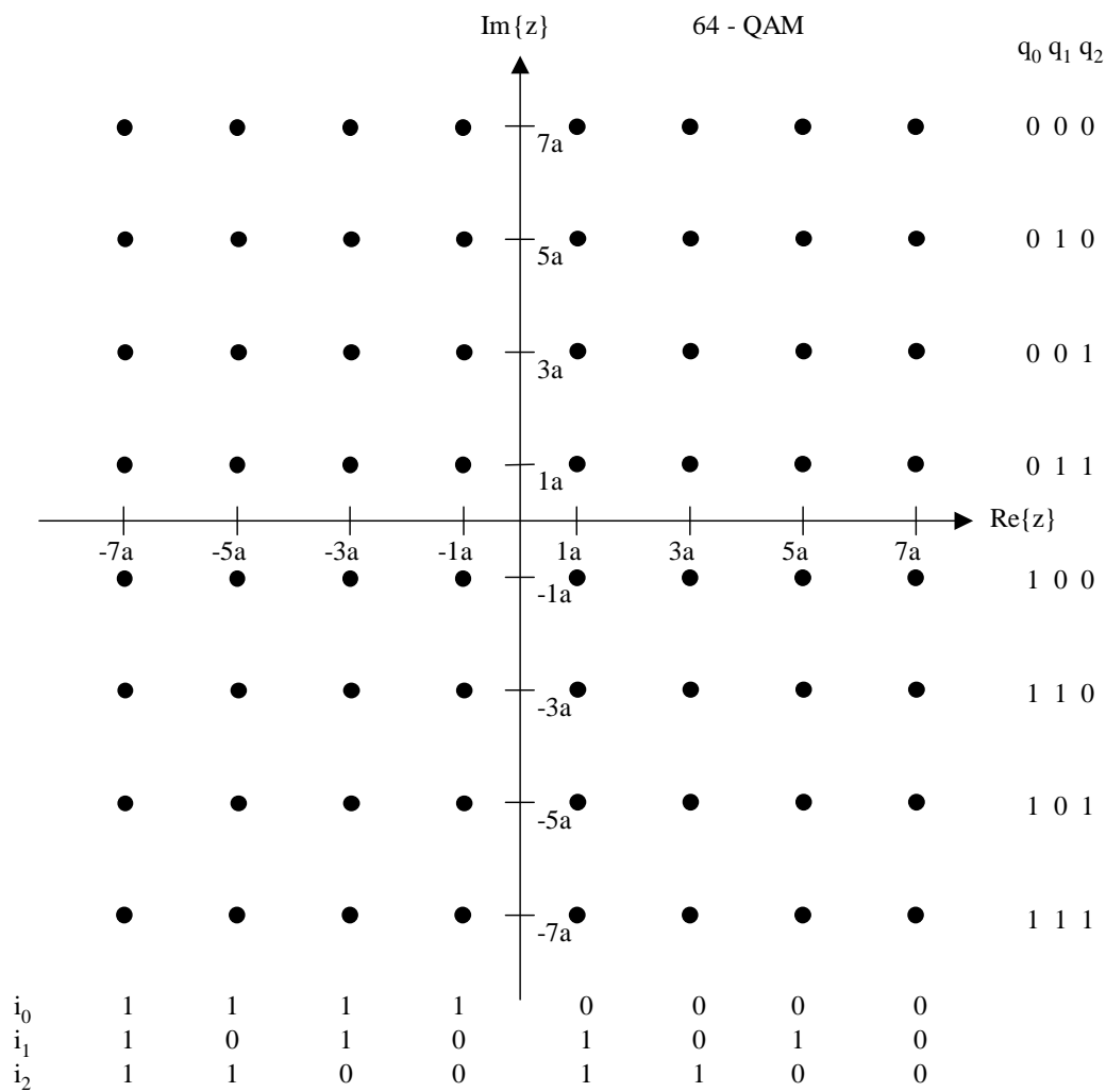
Figure 33: HMsym 64-QAM mapping with corresponding bit pattern
