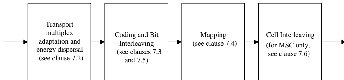
Figure 24: Functional block diagram of the coding and interleaving
