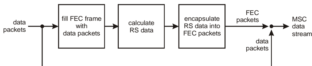
Figure 18: Conceptual diagram of the outer coder and outer interleaver (encoder view)
