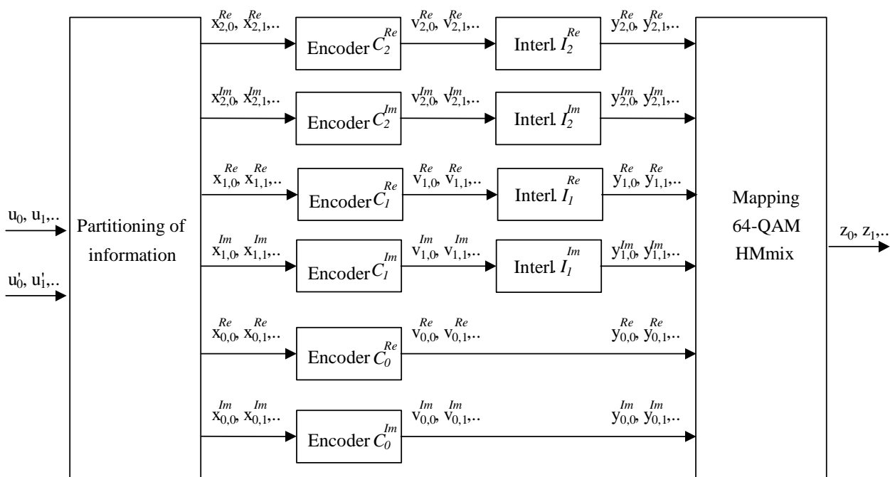
Figure 28: Multilevel coding with 3 levels for HMix
