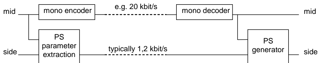
Figure 16: Topology of a codec system using parametric stereo
