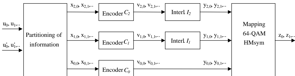
Figure 27: Multilevel coding with 3 levels for HMsym
