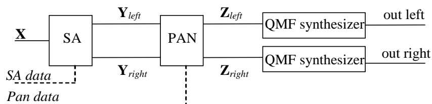
Figure 17: PS decoder module overview
