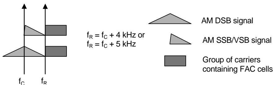
Figure K.3: Example simulcast modes for half channel offsets
