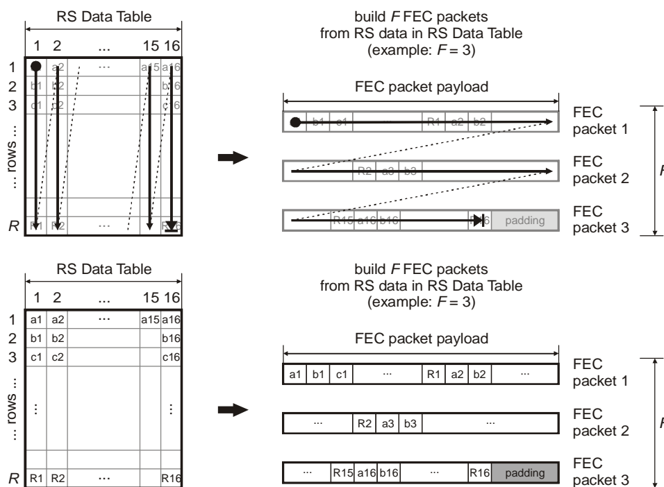
Figure 22: RS data byte order within FEC packets
