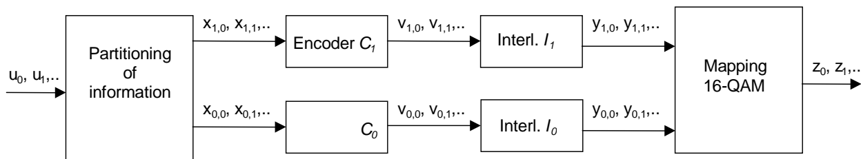
Figure 29: Multilevel coding with 2 levels (SM)
