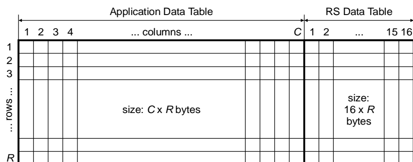
Figure 19: Structure of the FEC frame
