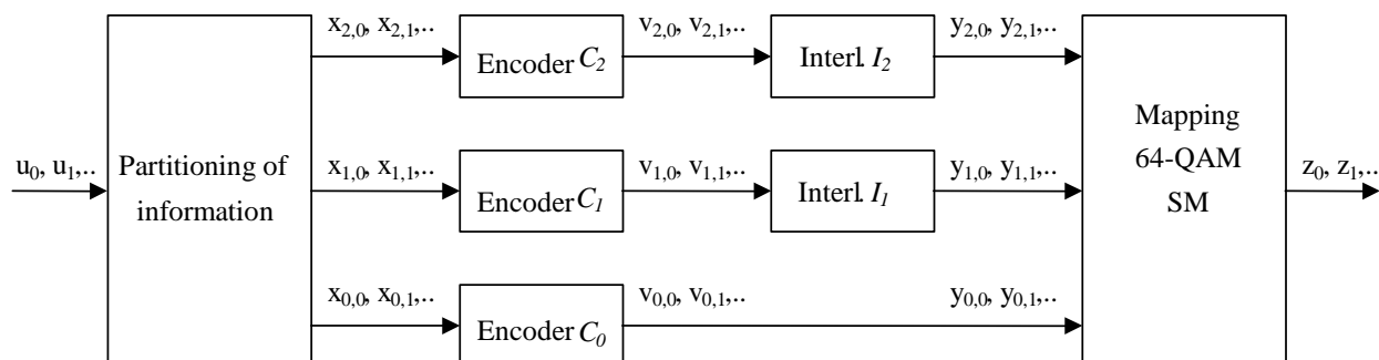
Figure 26: Multilevel coding with 3 levels for SM
