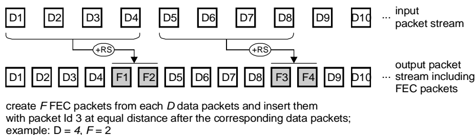
Figure 23: Inserting FEC packets into the packet stream
