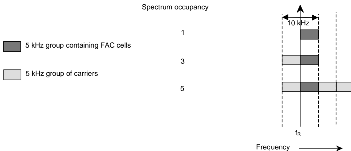
Figure 38: Spectrum occupancy for 10 kHz channels
