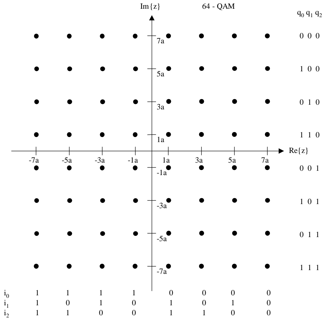
Figure 34: HMmix 64-QAM mapping with corresponding bit pattern
