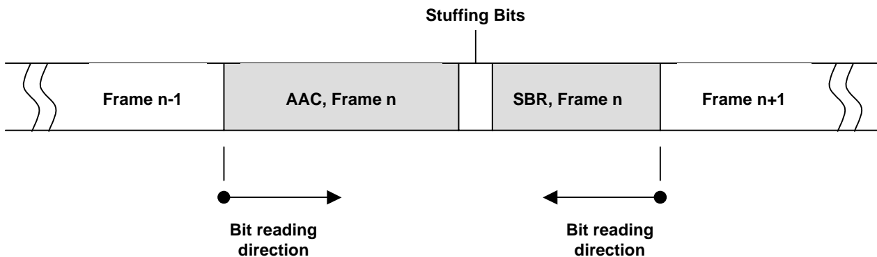
Figure 4: AAC + SBR frame
