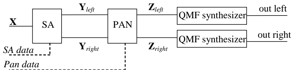
Figure 16: PS decoder module overview
