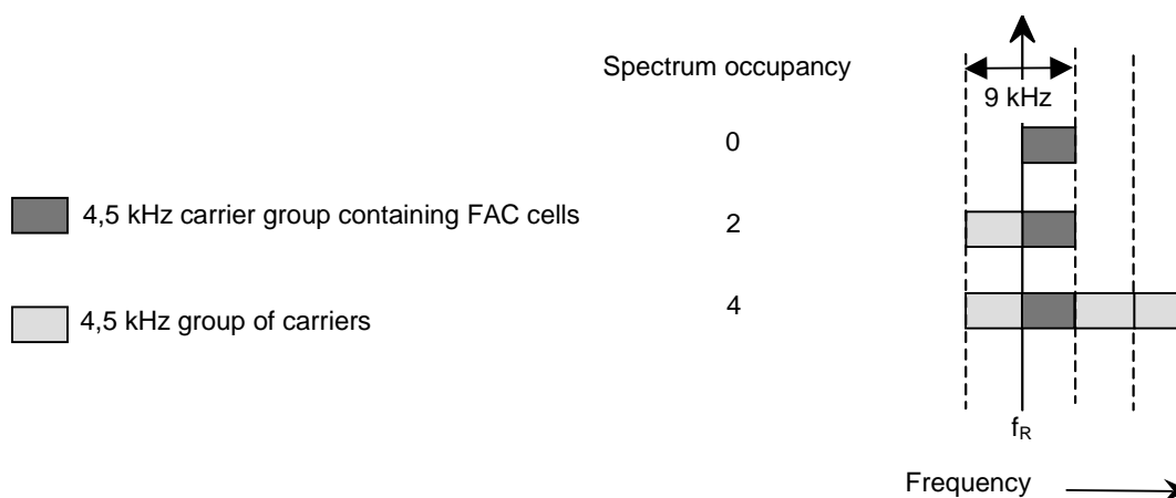
Figure 30: Spectrum occupancy for 9 kHz channels
