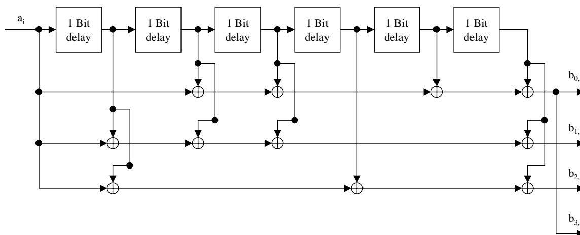
Figure 24: Convolutional encoder
