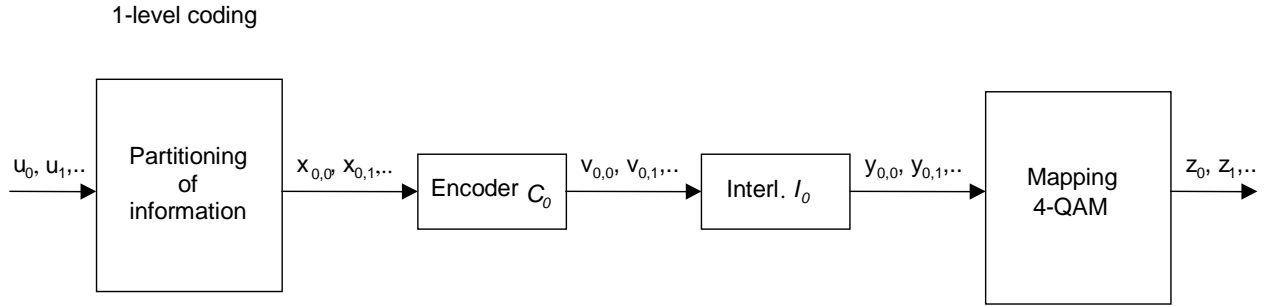
Figure 23: Multilevel coding with 1 level (SM)
