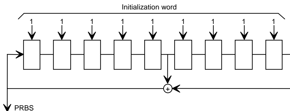
Figure 18: PRBS generator
