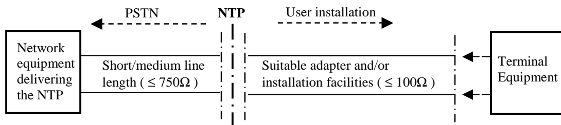
Figure 1: Network Termination Point (NTP)
