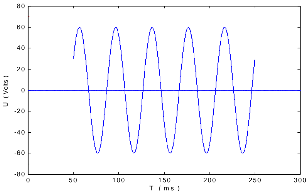
Figure 5: Example of the principle of switching the ringing voltage on and off at the right moment
