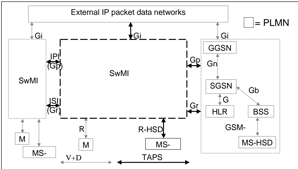
Figure 1: TAPS Interfaces
